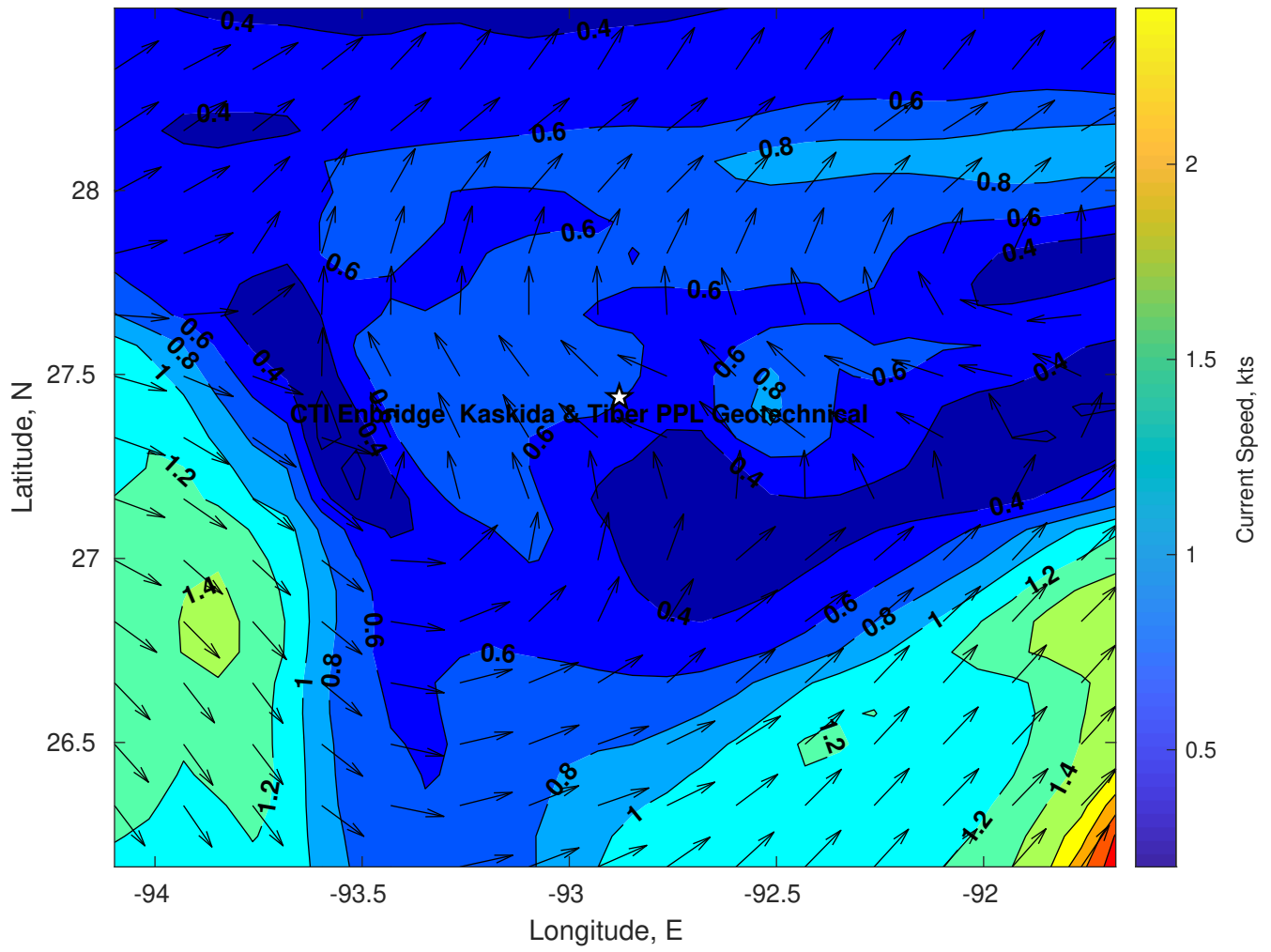
Surface Currents for CTI Enbridge Kaskida & Tiber PPL Geotechnical at 16-Feb-2025 00:00:00
