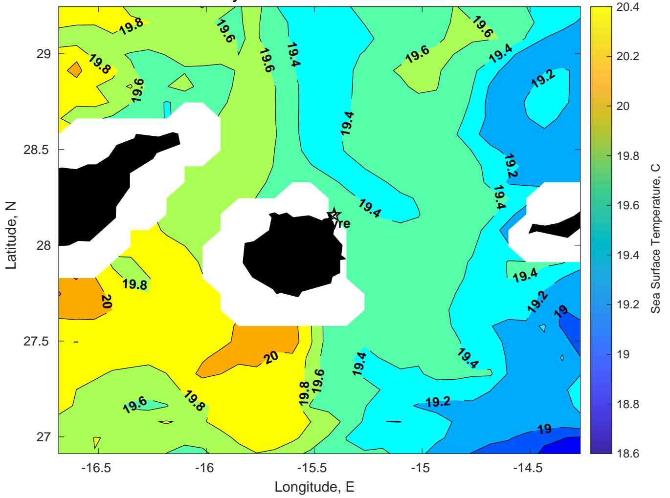
SST for Gyre at 16-Feb-2025 00:00:00
