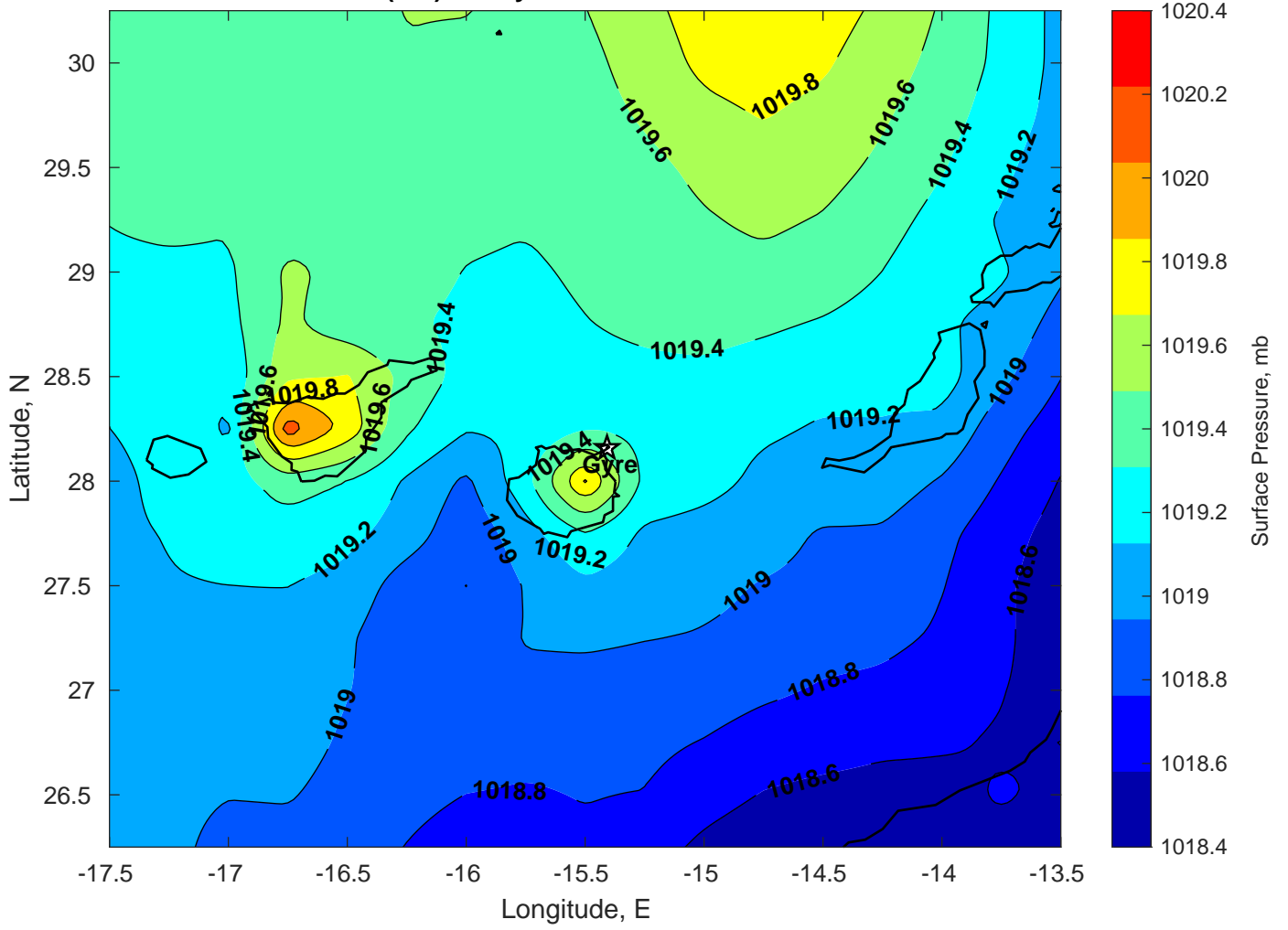
Surface Pressure (mb) for Gyre at 17-Feb-2025 00:00:00
