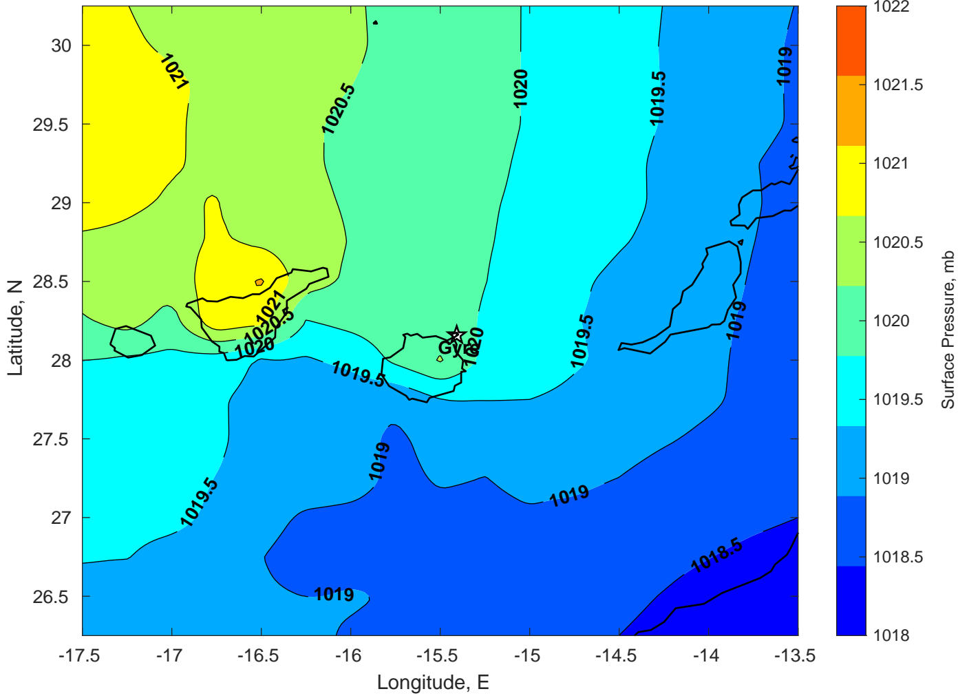
Surface Pressure (mb) for Gyre at 19-Feb-2025 00:00:00
