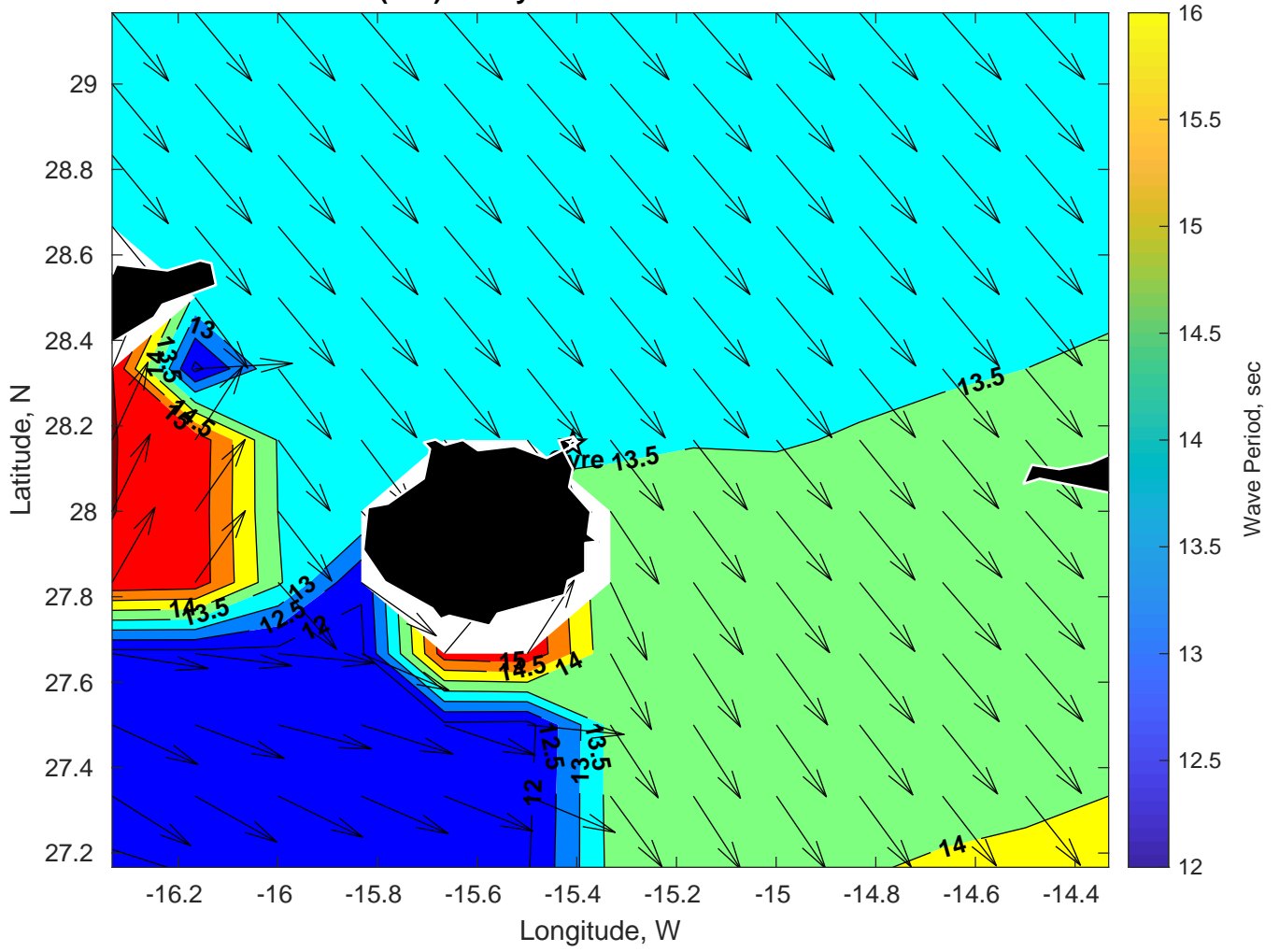
Wave Period (sec) for Gyre at 17-Feb-2025 09:00:00
