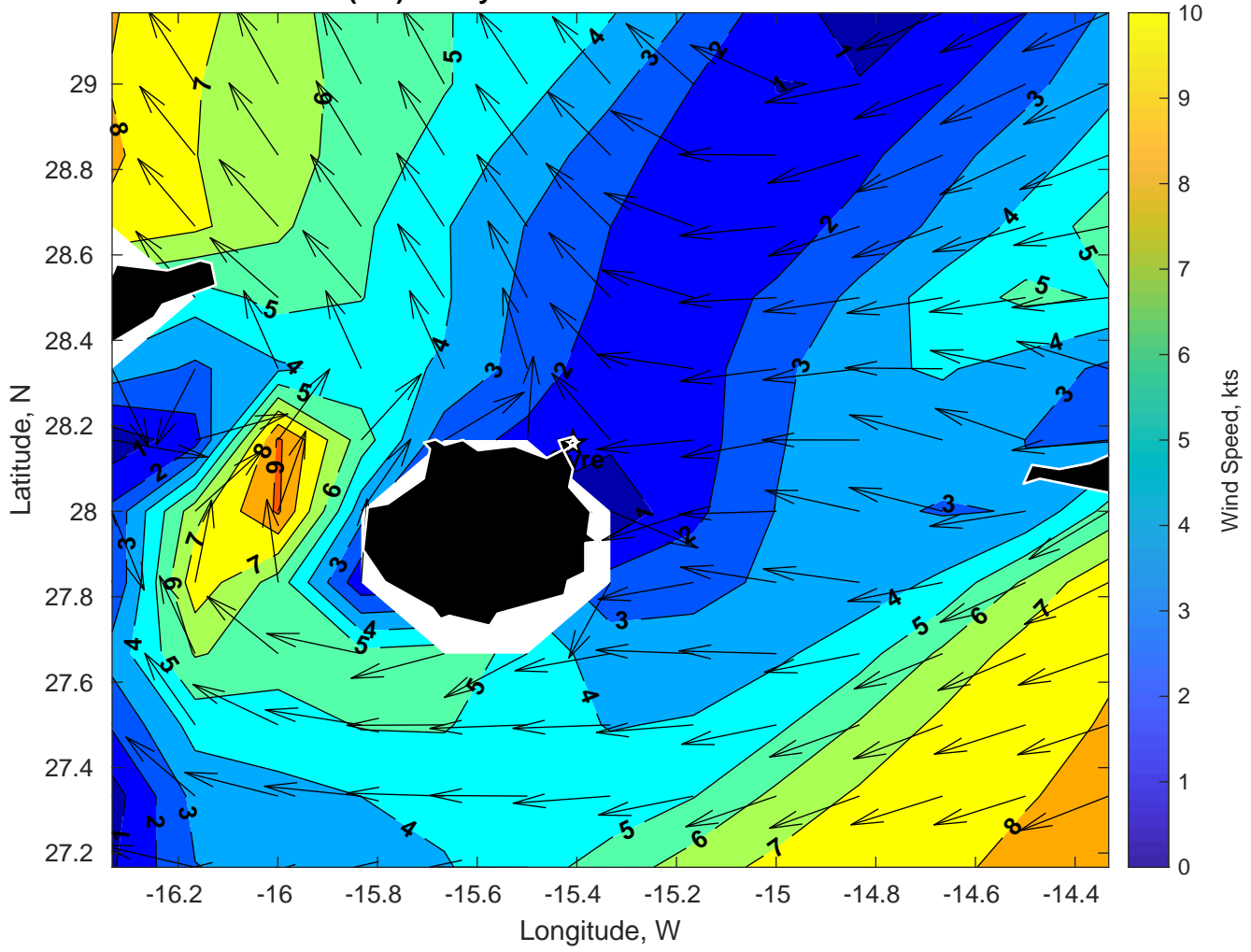
Winds (kts) for Gyre at 17-Feb-2025 09:00:00
