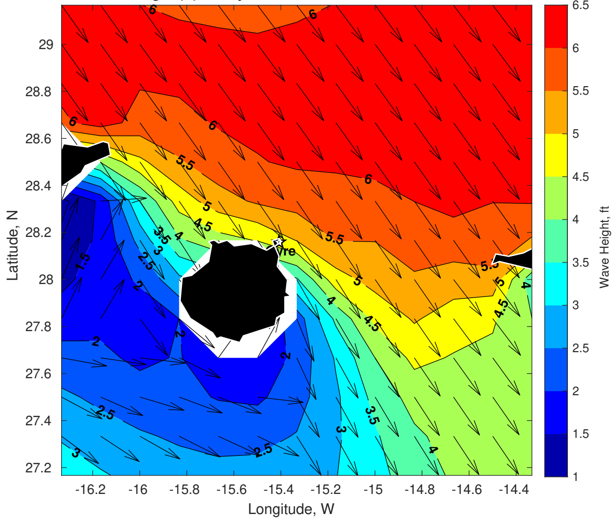
Wave Height (ft) for Gyre at 17-Feb-2025 09:00:00
