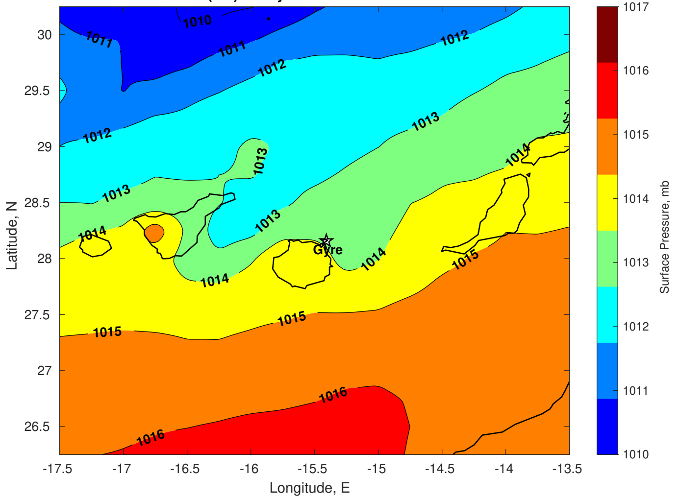
Surface Pressure (mb) for Gyre at 18-Feb-2025 00:00:00
