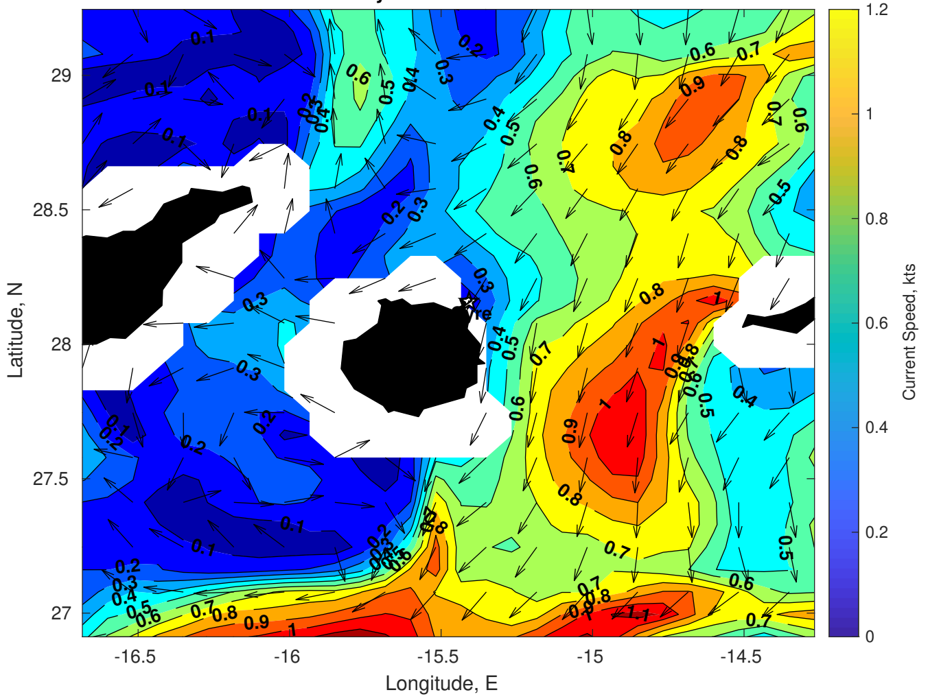
Surface Currents for Gyre at 16-Feb-2025 00:00:00
