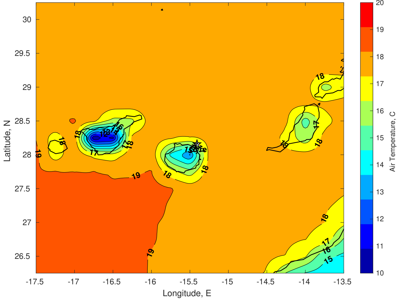
Air Temperature (C) for Gyre at 17-Feb-2025
