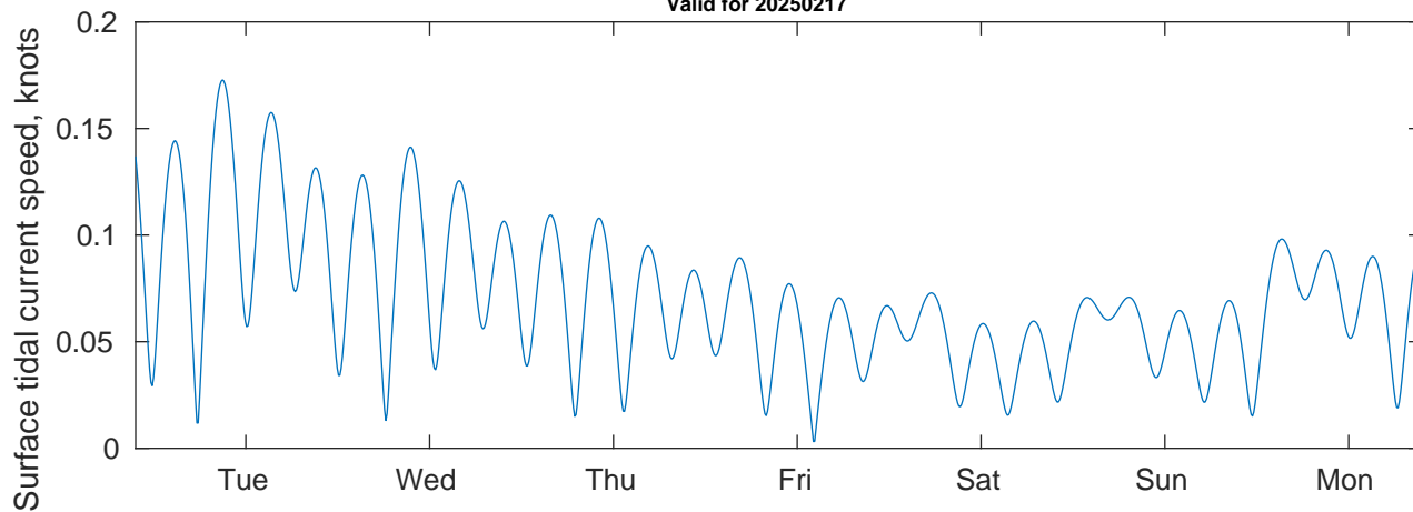
Tidal Currents and Heights for Gyre at 20250217
