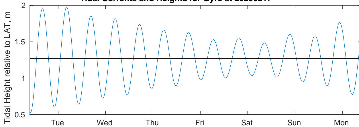
Tidal Currents and Heights for Gyre at 20250217
