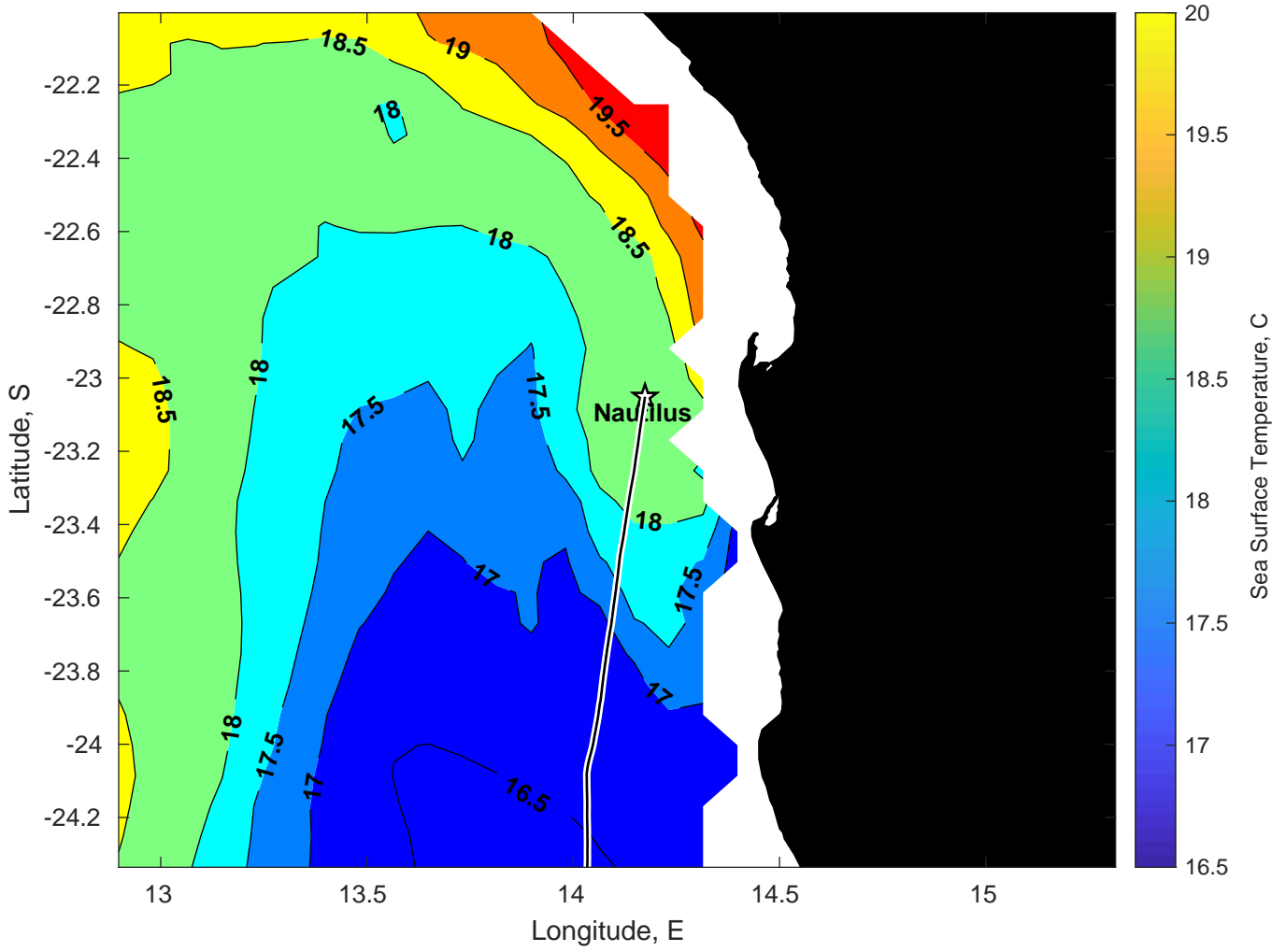
SST for Nautilus at 16-Feb-2025 00:00:00
