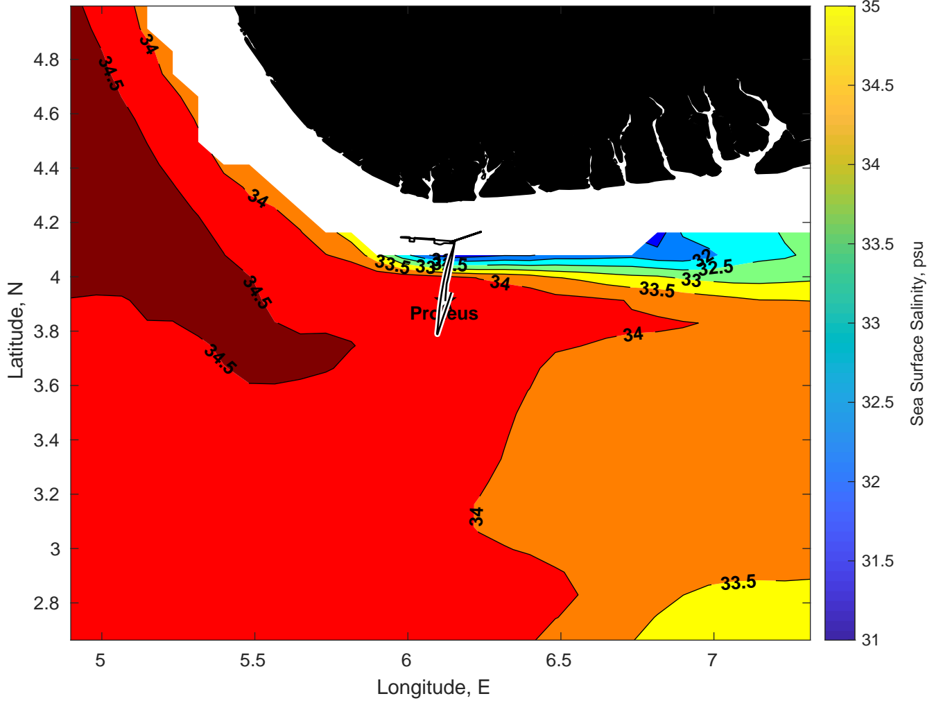
Surface Salinity for Proteus at 16-Feb-2025 00:00:00
