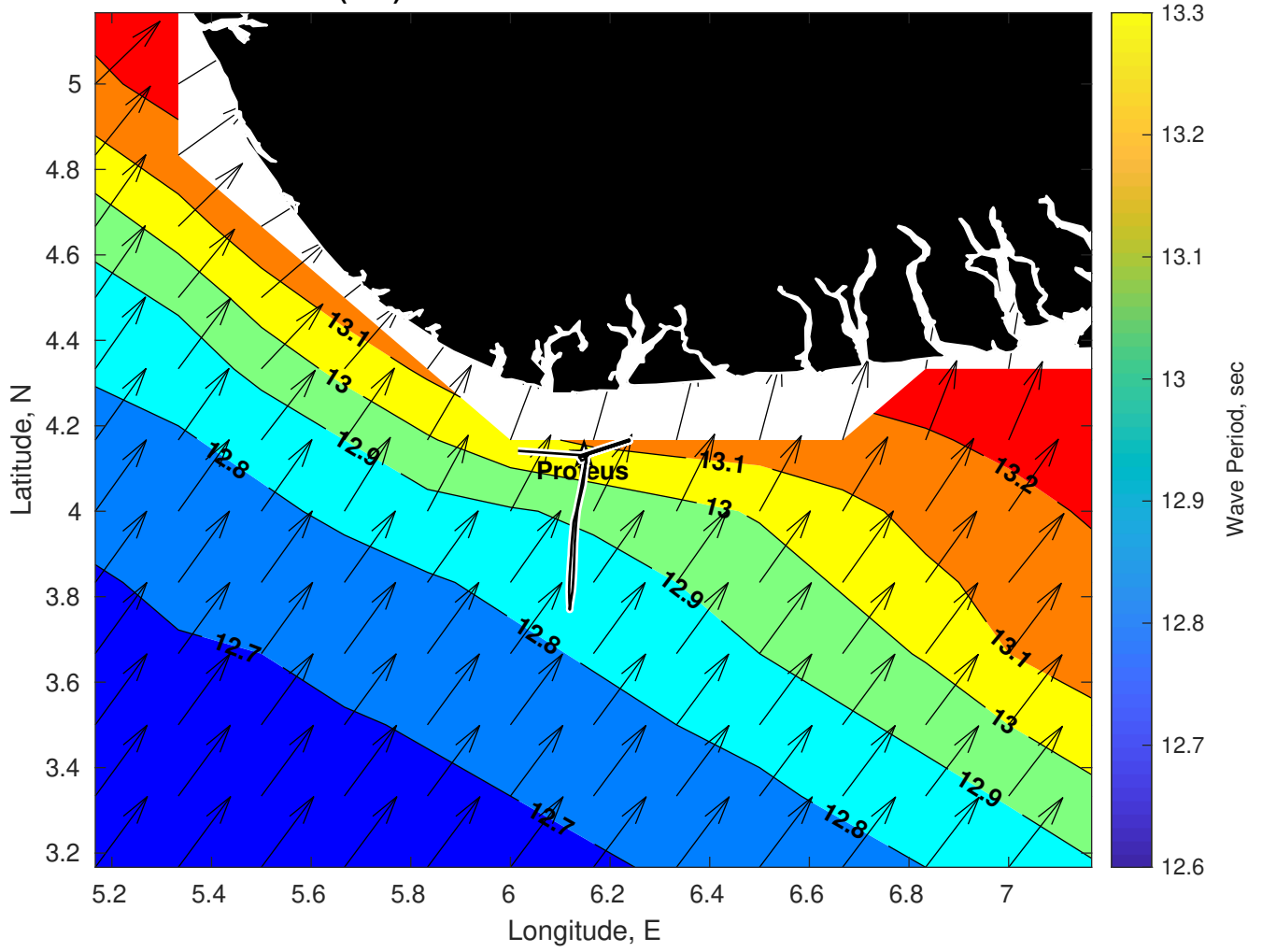
Wave Period (sec) for Proteus at 17-Feb-2025 09:00:00
