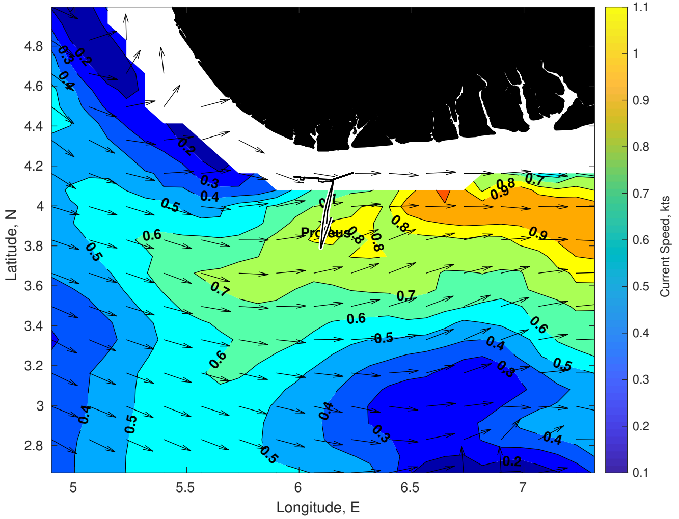
Surface Currents for Proteus at 16-Feb-2025 00:00:00
