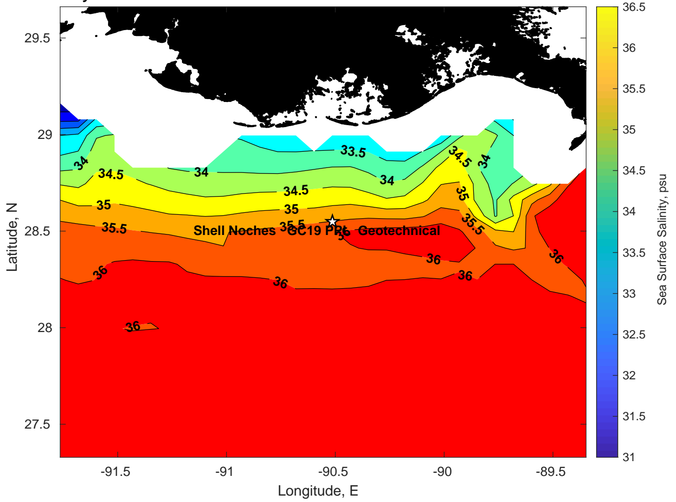
Surface Salinity for Shell Noches GC19 PPL Geotechnical at 16-Feb-2025 00:00:00
