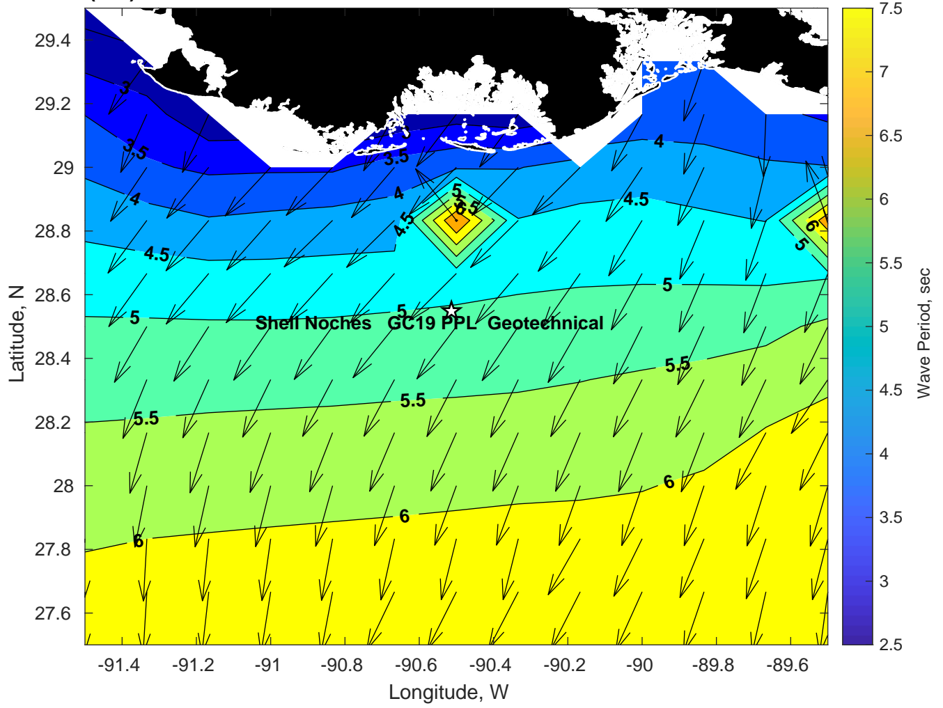
Wave Period (sec) for Shell Noches GC19 PPL Geotechnical at 17-Feb-2025 09:00:00
