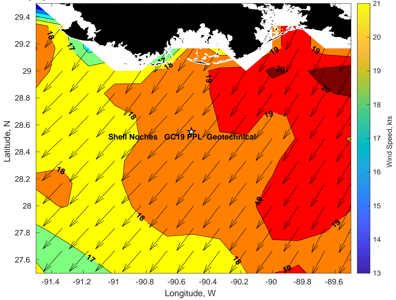
Winds (kts) for Shell Noches GC19 PPL Geotechnical at 17-Feb-2025 09:00:00
