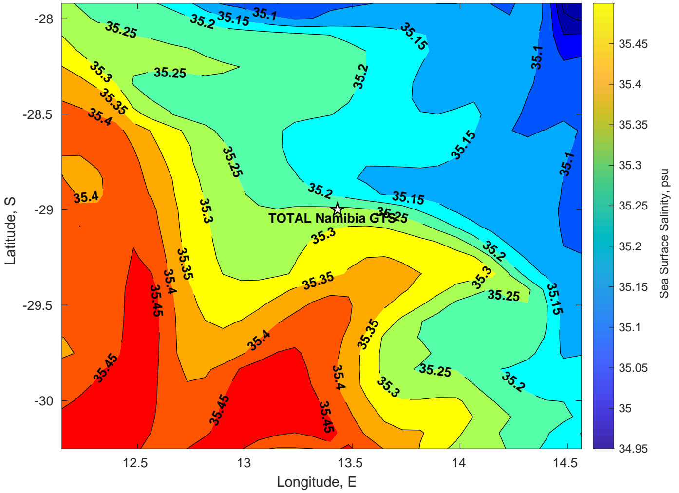
Surface Salinity for TOTAL Namibia GTS at 16-Feb-2025 00:00:00
