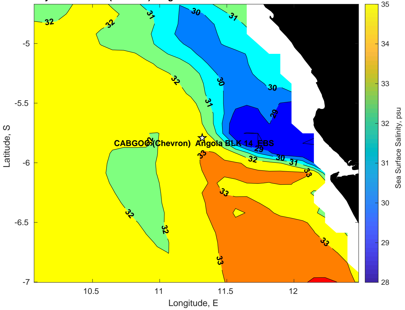
Surface Salinity for CABGOC (Chevron) Angola BLK 14 EBS at 17-Feb-2025 00:00:00
