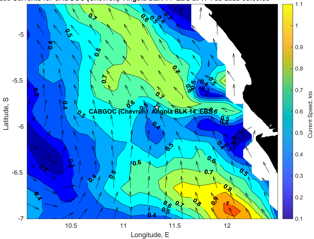
Surface Currents for CABGOC (Chevron) Angola BLK 14 EBS at 17-Feb-2025 00:00:00
