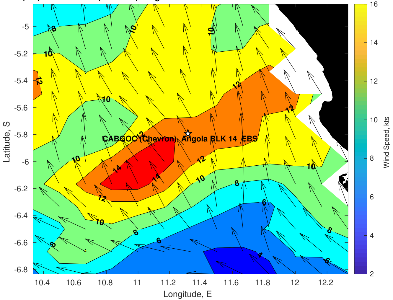
Winds (kts) for CABGOC (Chevron) Angola BLK 14 EBS at 18-Feb-2025 09:00:00
