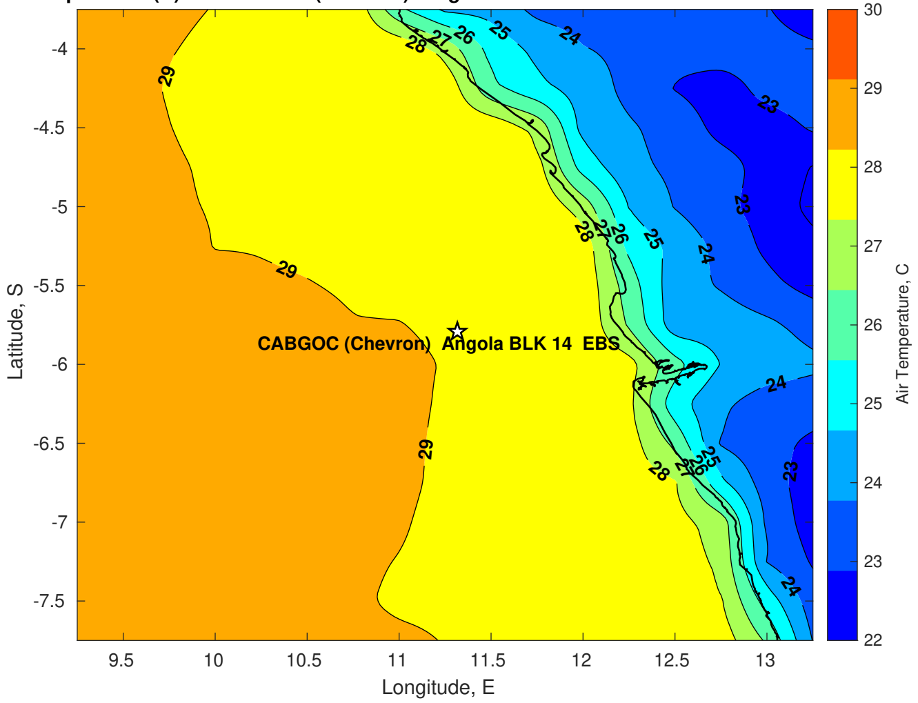
Air Temperature (C) for CABGOC (Chevron) Angola BLK 14 EBS at 18-Feb-2025
