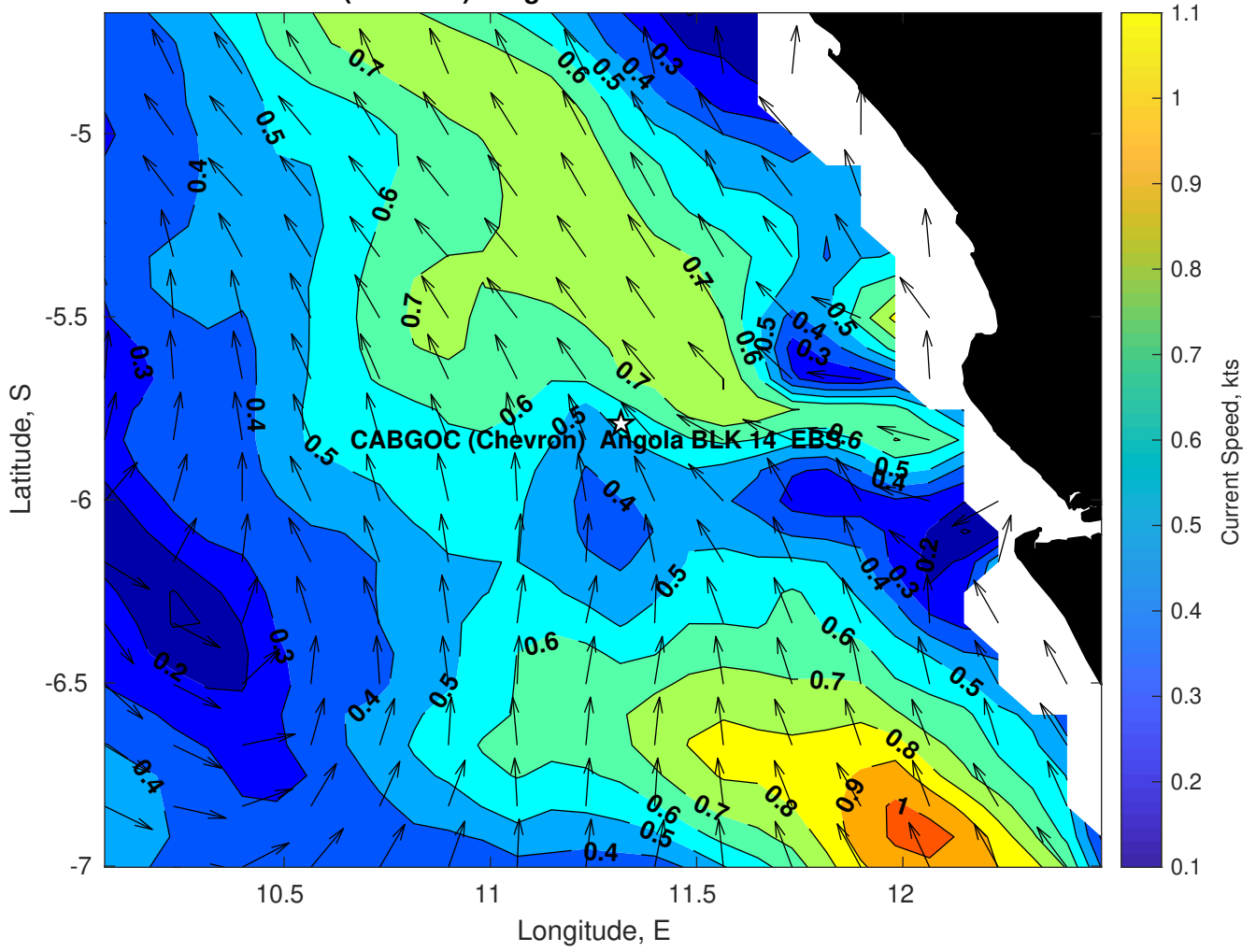
Surface Currents for CABGOC (Chevron) Angola BLK 14 EBS at 17-Feb-2025 00:00:00
