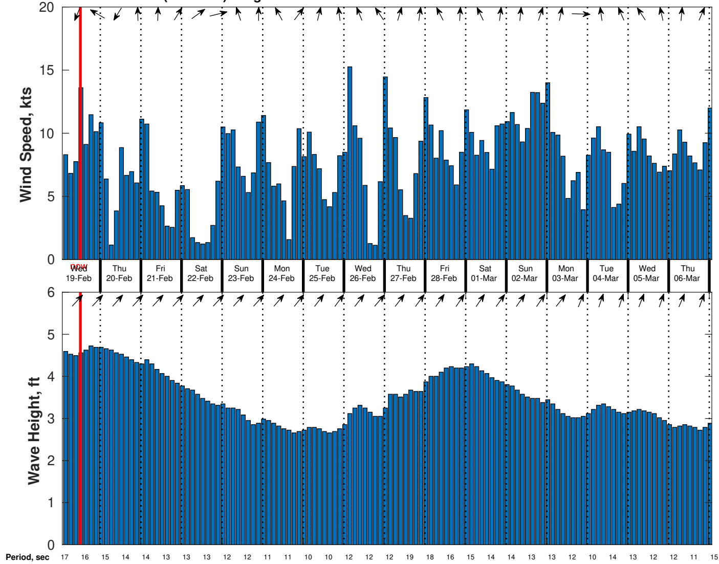
Wind & Wave Forecast for CABGOC (Chevron) Angola BLK 14 EBS from 18-Feb-2025 02:00:00 to 06-Mar-2025 02:00:00
