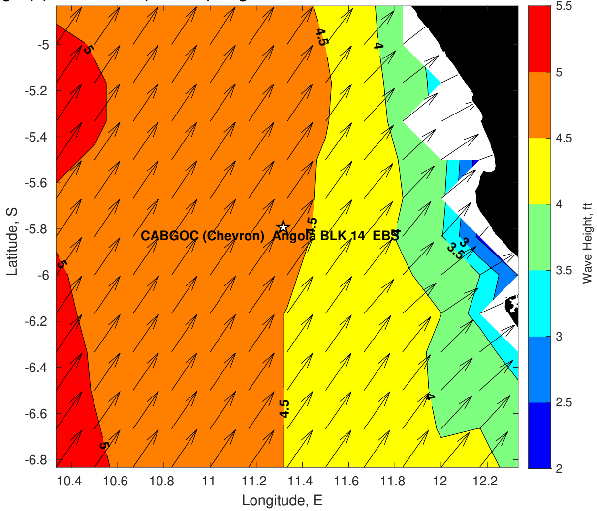
Wave Height (ft) for CABGOC (Chevron) Angola BLK 14 EBS at 18-Feb-2025 09:00:00
