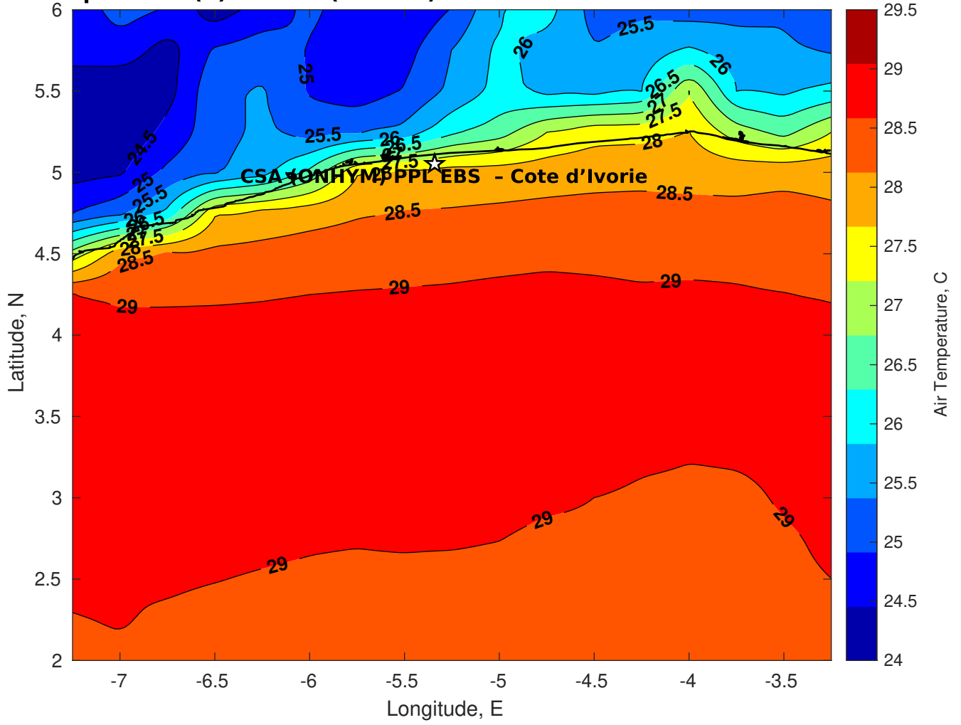
Air Temperature (C) for CSA (ONHYM) PPL EBS - Cote d'Ivoire at 18-Feb-2025
