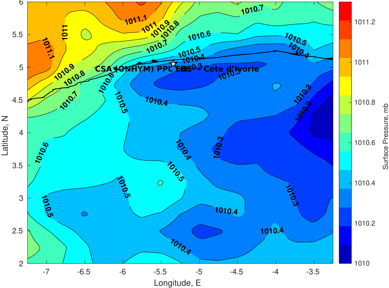
Surface Pressure (mb) for CSA (ONHYM) PPL EBS - Cote d'Ivoire at 20-Feb-2025 06:00:00
