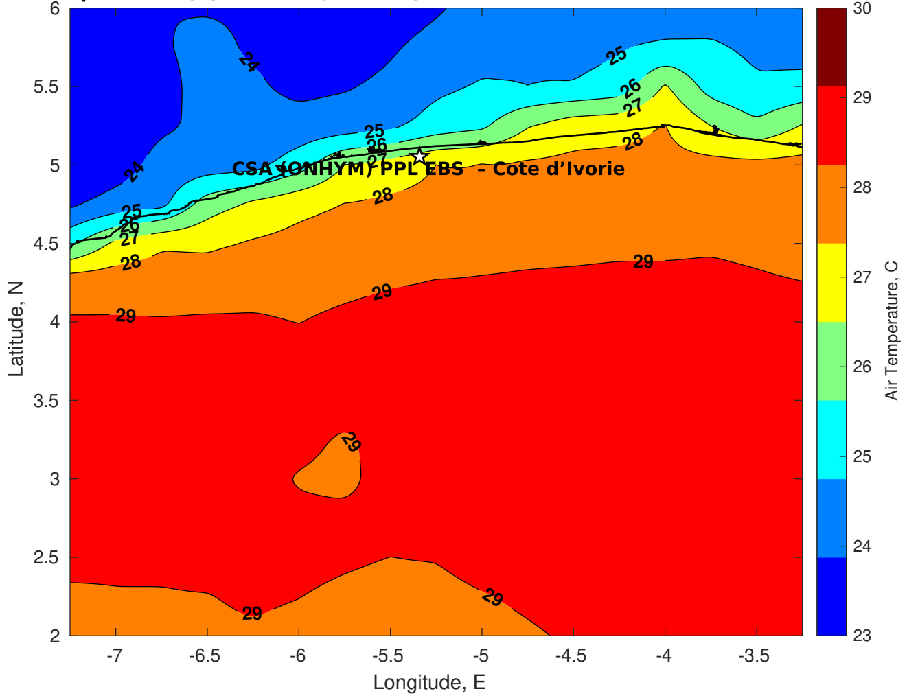
Air Temperature (C) for CSA (ONHYM) PPL EBS - Cote d'Ivoire at 18-Feb-2025
