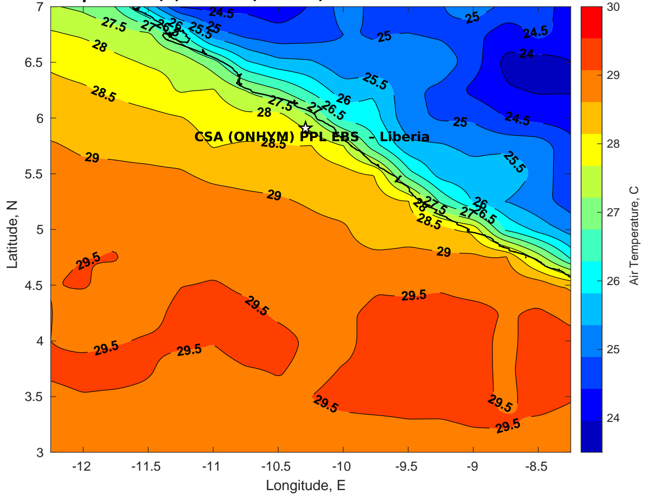
Air Temperature (C) for CSA (ONHYM) PPL EBS - Liberia at 18-Feb-2025
