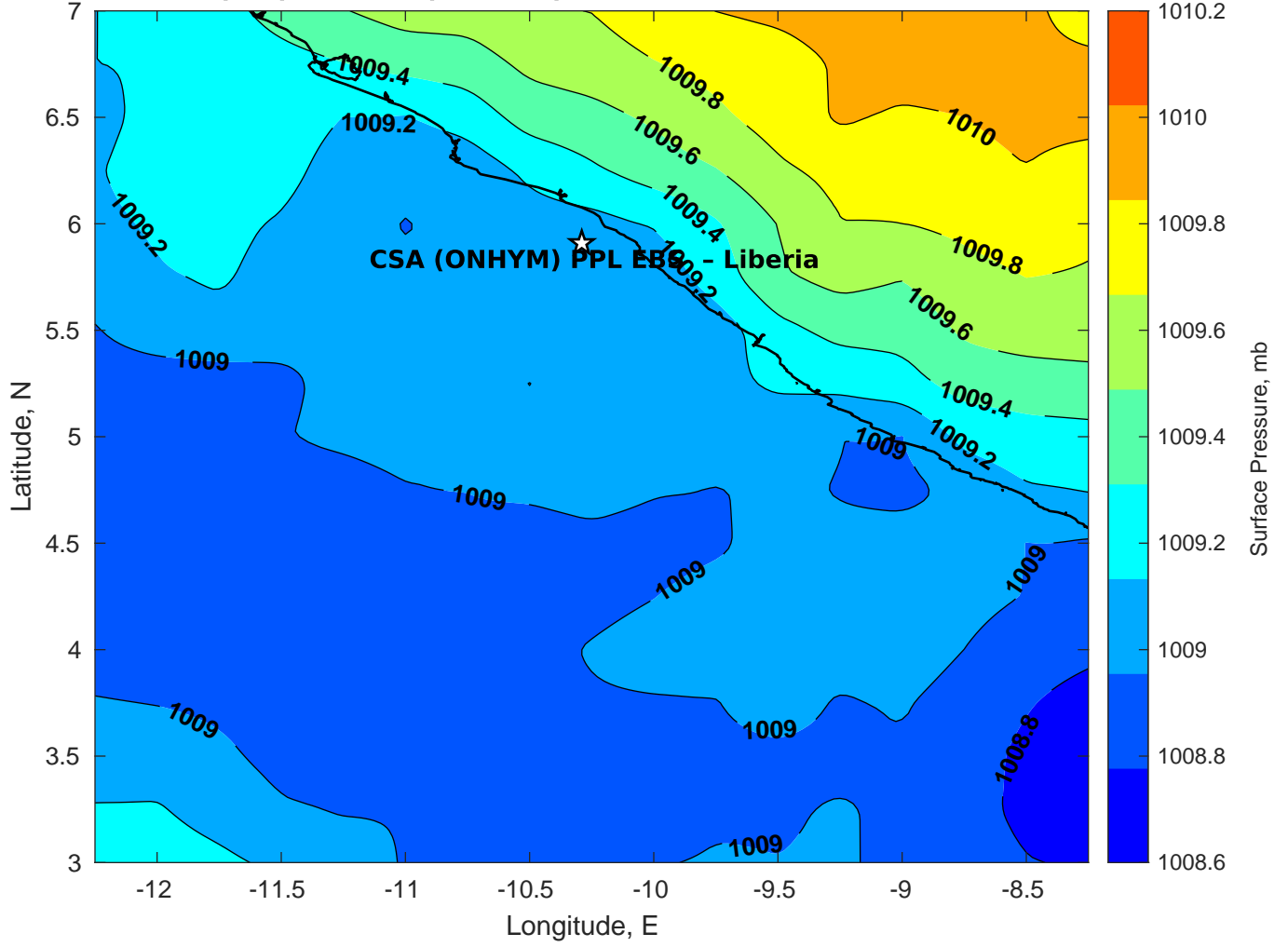
Surface Pressure (mb) for CSA (ONHYM) PPL EBS - Liberia at 18-Feb-2025 06:00:00
