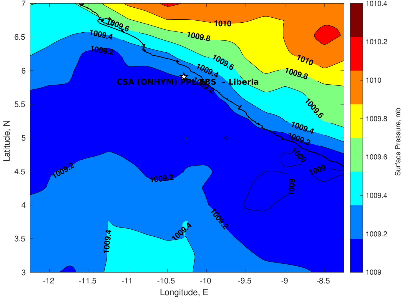
Surface Pressure (mb) for CSA (ONHYM) PPL EBS - Liberia at 19-Feb-2025 06:00:00
