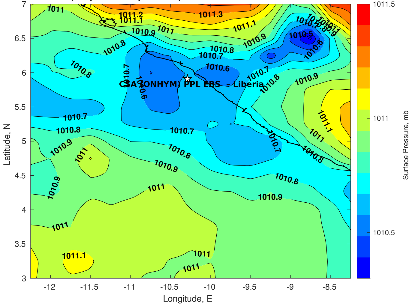
Surface Pressure (mb) for CSA (ONHYM) PPL EBS - Liberia at 20-Feb-2025 06:00:00
