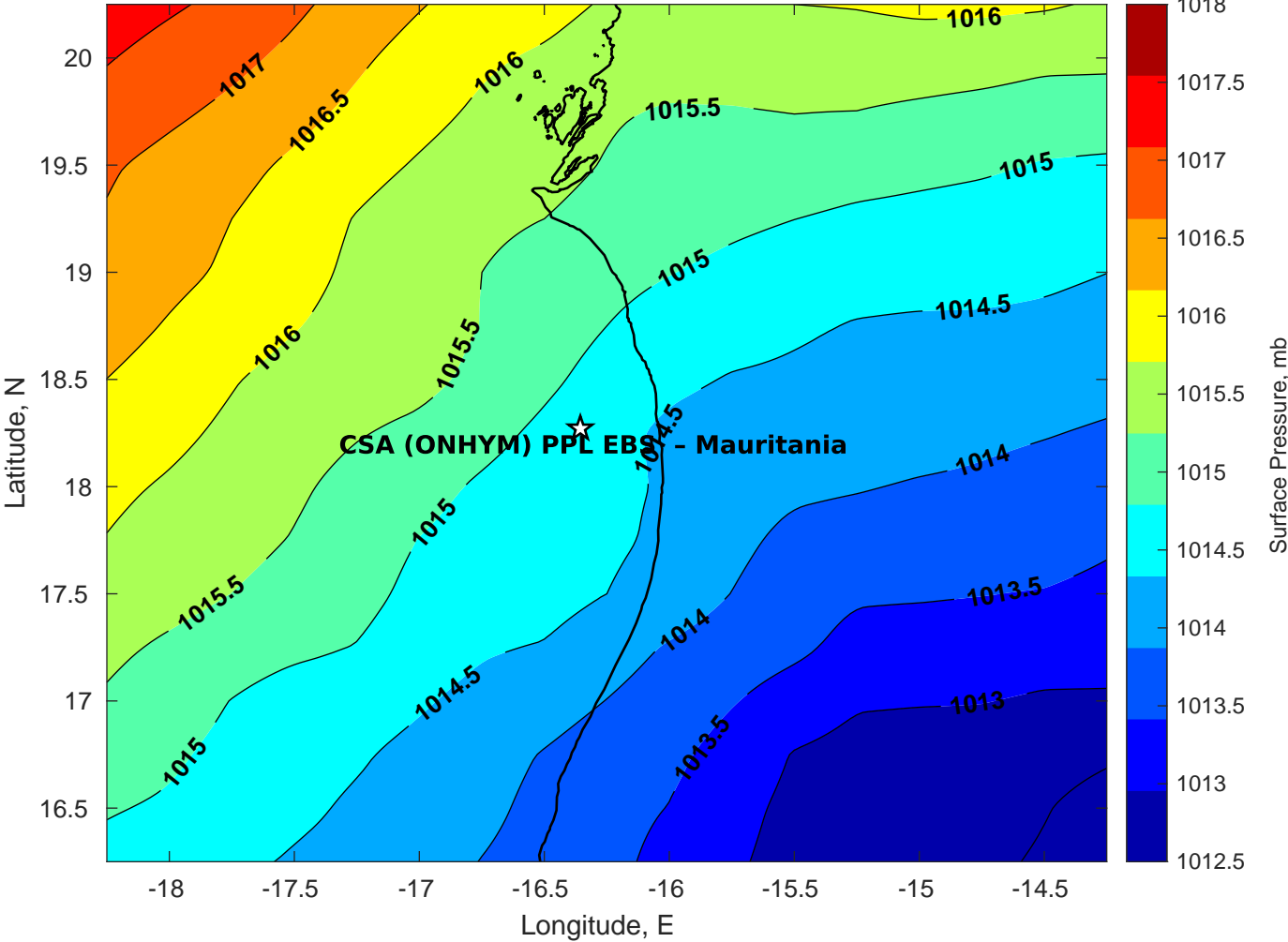
Surface Pressure (mb) for CSA (ONHYM) PPL EBS - Mauritania at 20-Feb-2025 00:00:00
