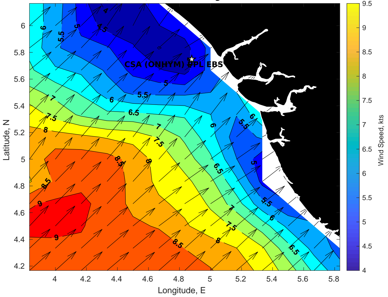
Winds (kts) for CSA (ONHYM) PPL EBS - Nigeria at 18-Feb-2025 09:00:00
