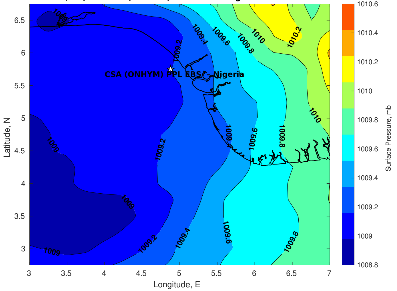
Surface Pressure (mb) for CSA (ONHYM) PPL EBS - Nigeria at 19-Feb-2025 06:00:00
