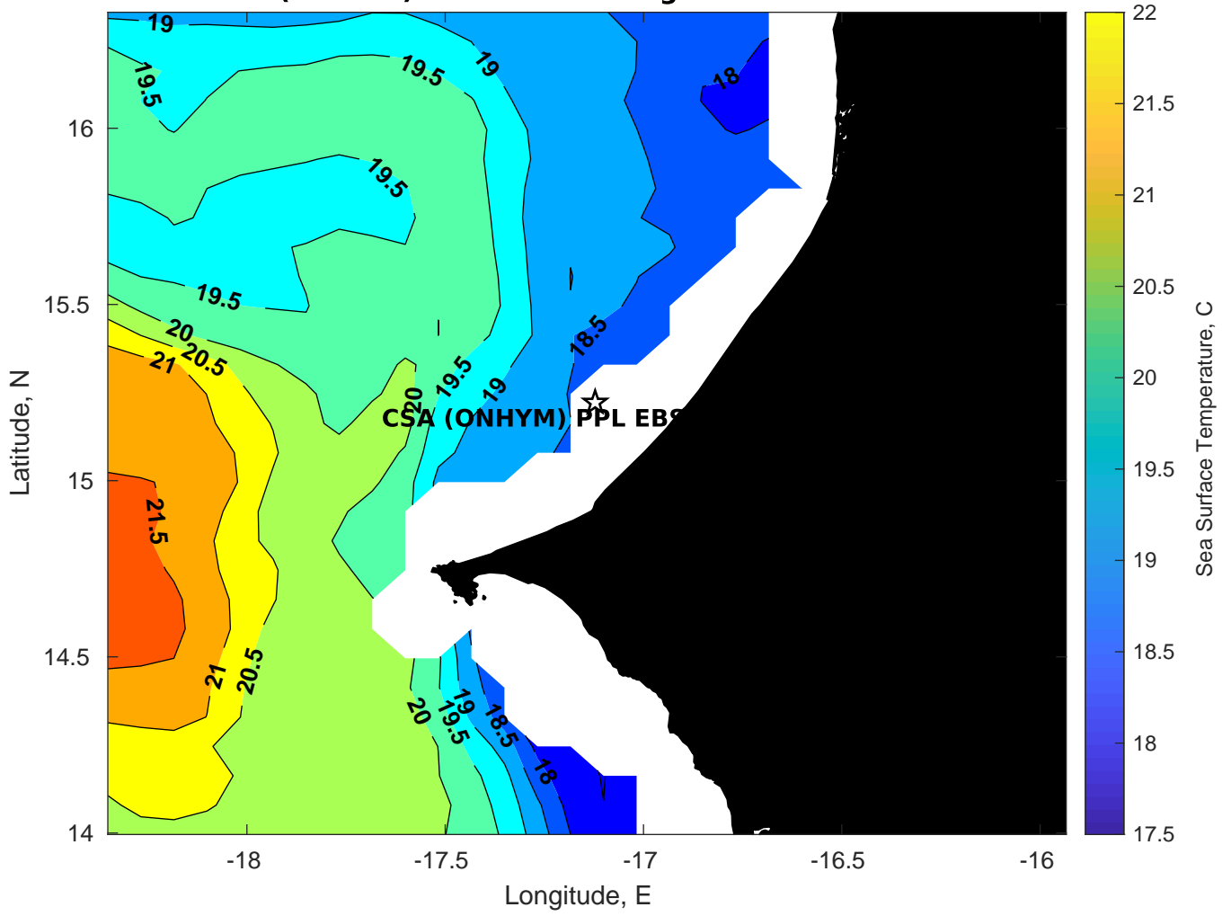
SST for CSA (ONHYM) PPL EBS - Senegal at 17-Feb-2025 00:00:00
