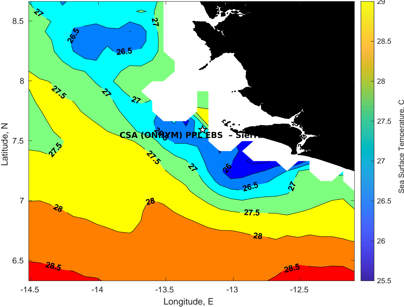
SST for CSA (ONHYM) PPL EBS - Sierra Leone at 17-Feb-2025 00:00:00
