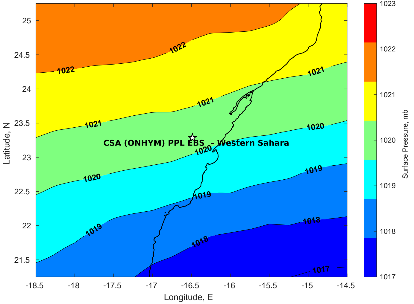
Surface Pressure (mb) for CSA (ONHYM) PPL EBS - Western Sahara at 20-Feb-2025 00:00:00
