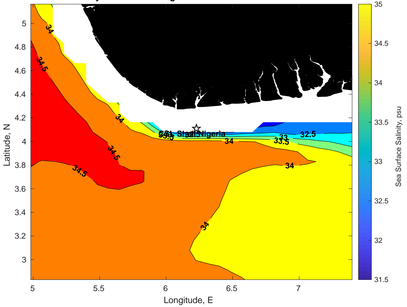
Surface Salinity for CSL Shell Nigeria at 17-Feb-2025 00:00:00
