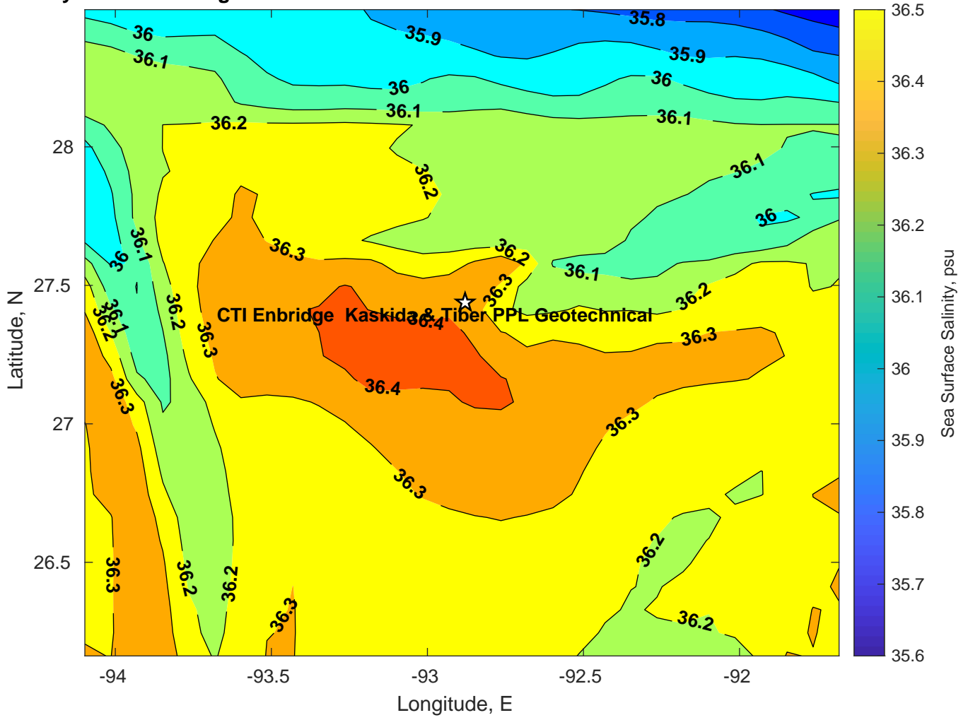
Surface Salinity for CTI Enbridge Kaskida & Tiber PPL Geotechnical at 17-Feb-2025 00:00:00
