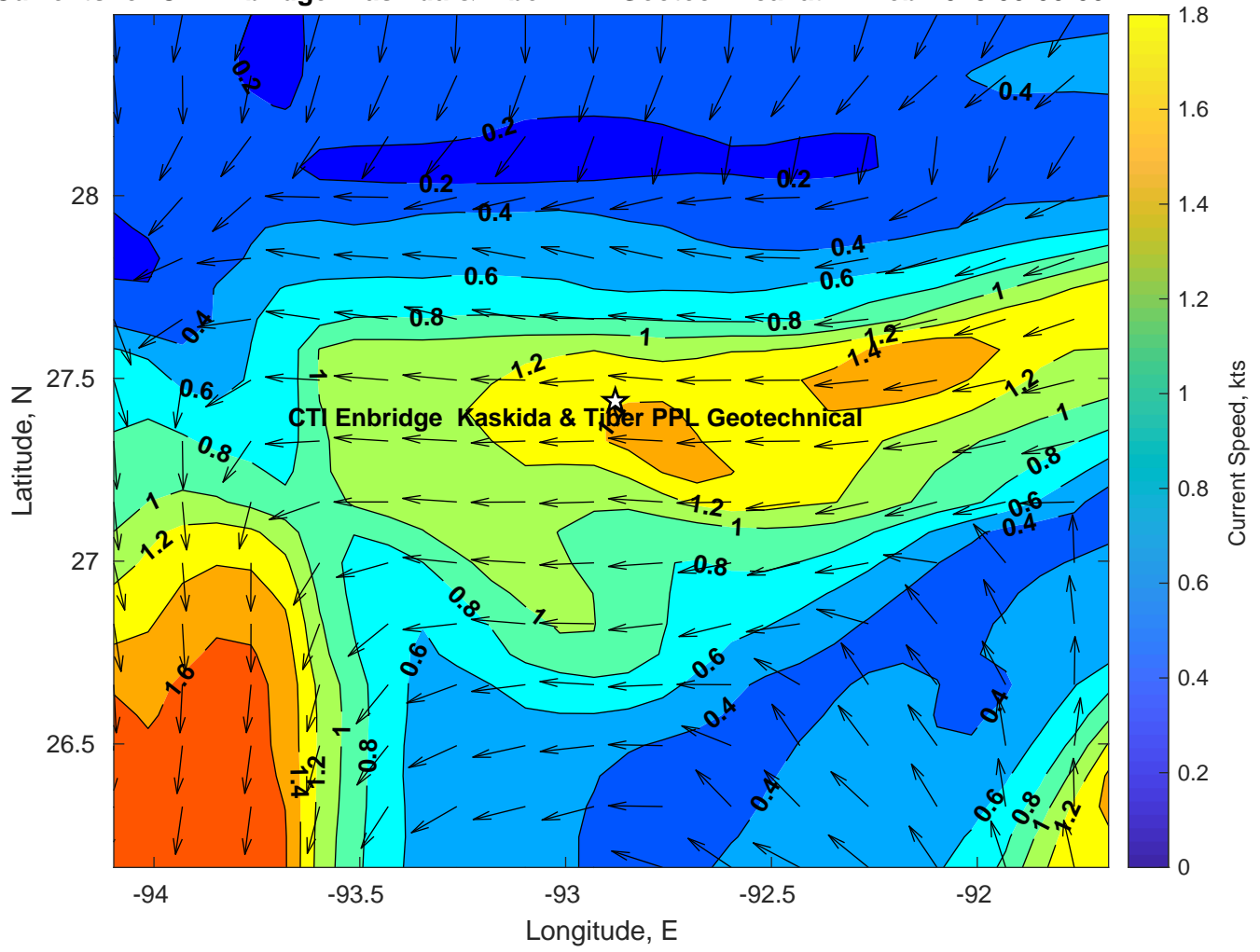
Surface Currents for CTI Enbridge Kaskida & Tiber PPL Geotechnical at 17-Feb-2025 00:00:00
