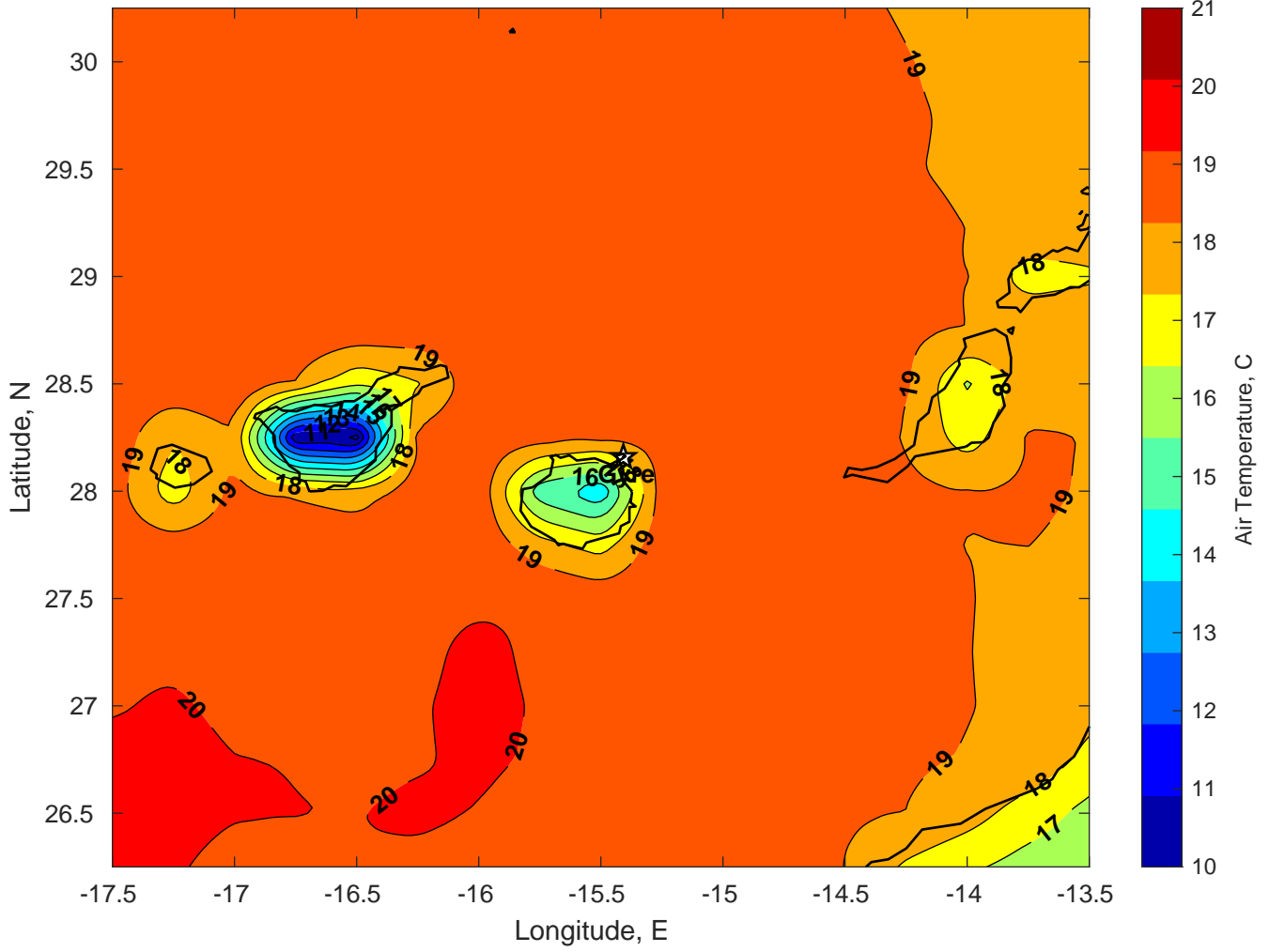
Air Temperature (C) for Gyre at 18-Feb-2025
