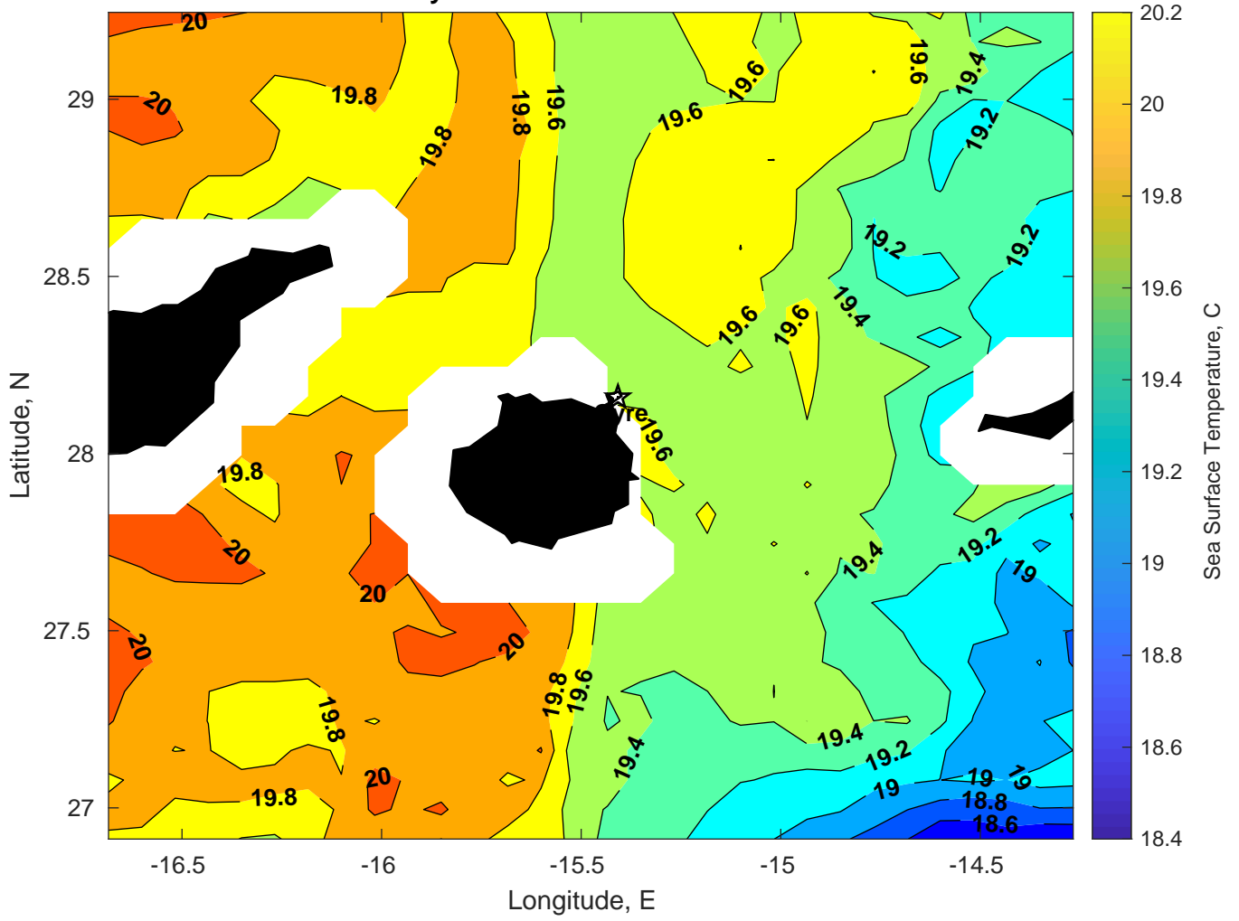
SST for Gyre at 17-Feb-2025 00:00:00
