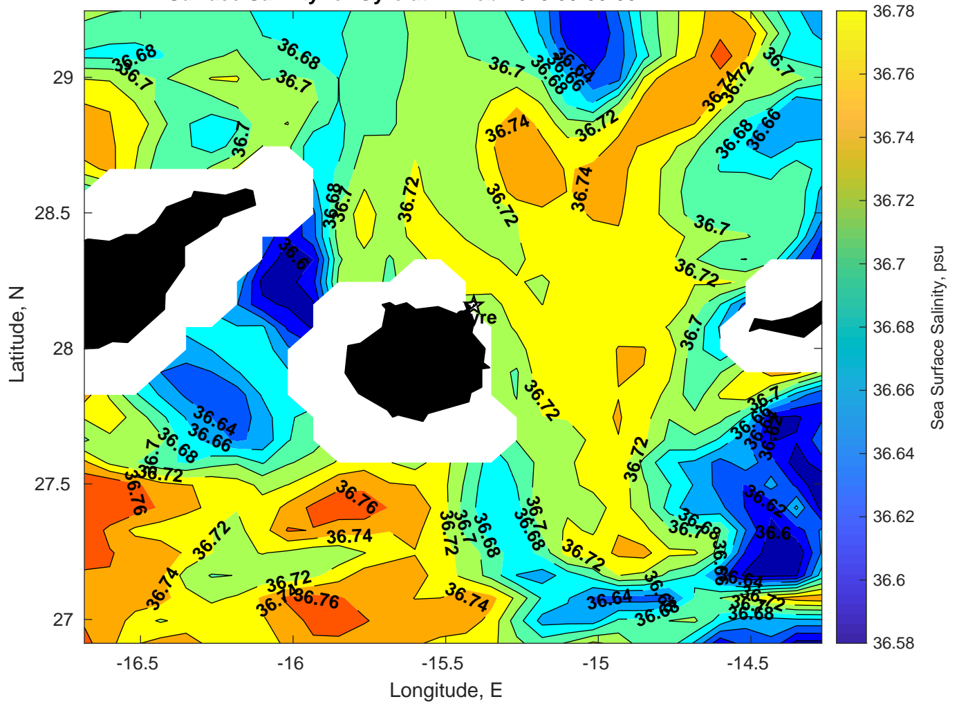
Surface Salinity for Gyre at 17-Feb-2025 00:00:00
