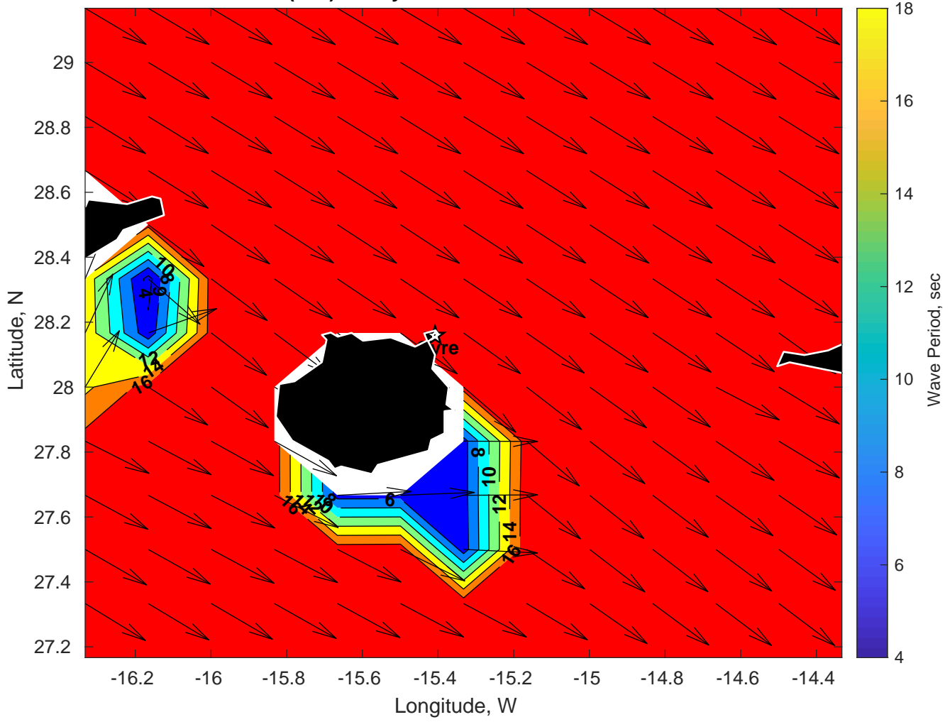
Wave Period (sec) for Gyre at 18-Feb-2025 09:00:00
