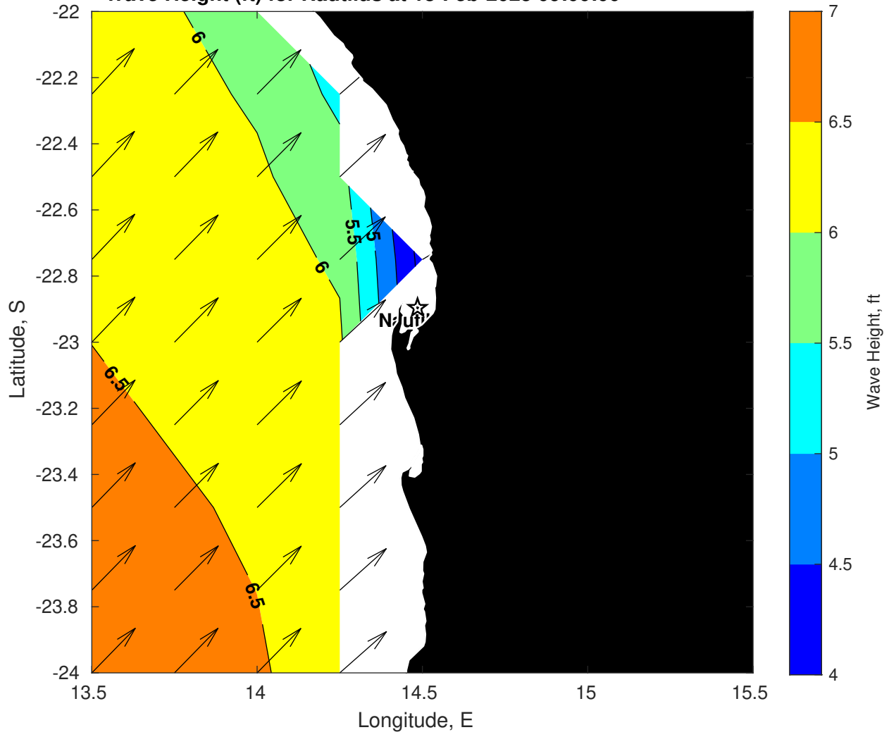
Wave Height (ft) for Nautilus at 18-Feb-2025 09:00:00
