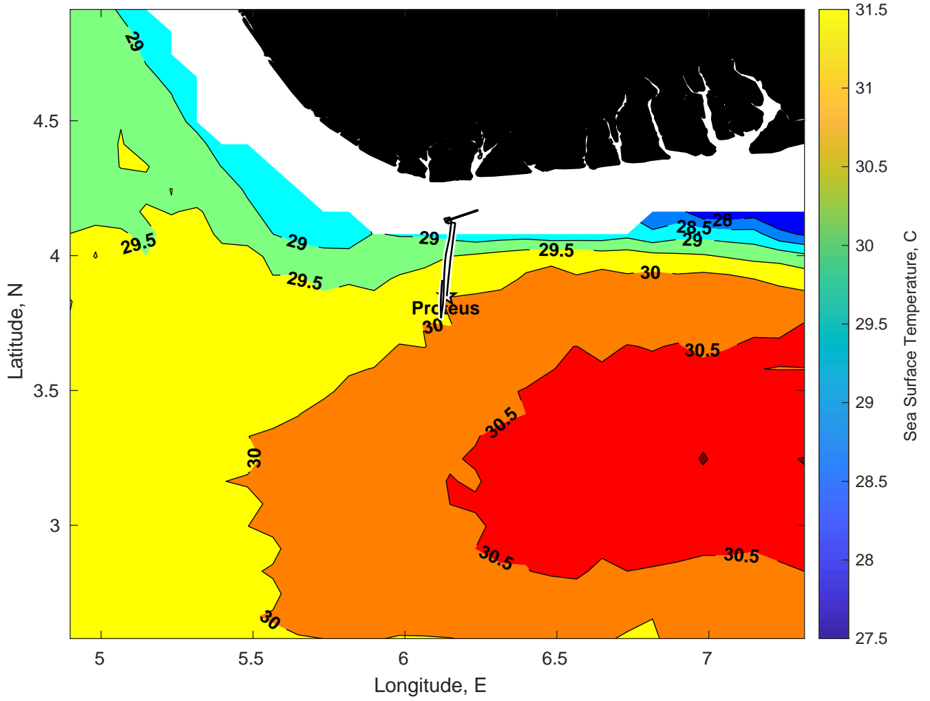
SST for Proteus at 17-Feb-2025 00:00:00
