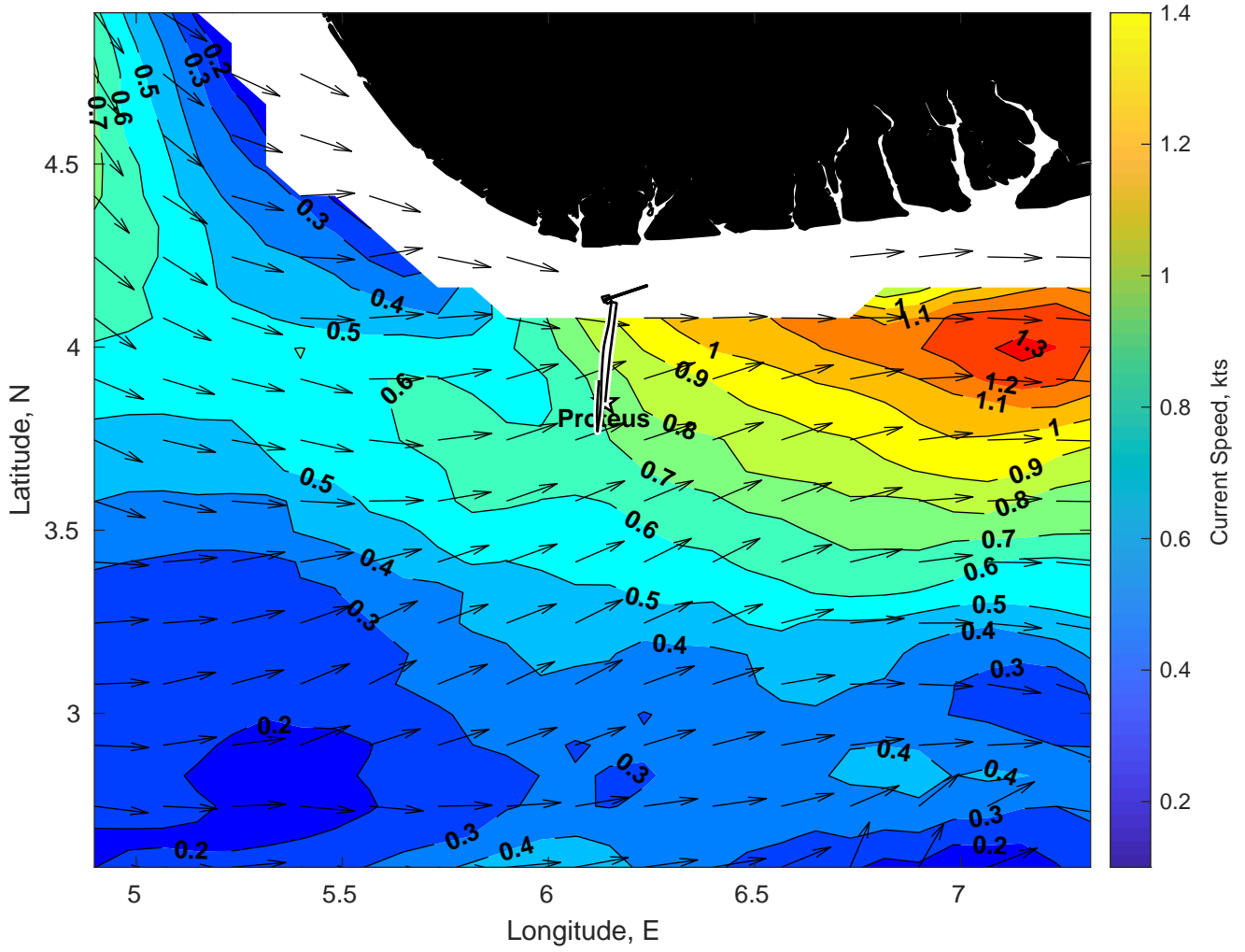
Surface Currents for Proteus at 17-Feb-2025 00:00:00
