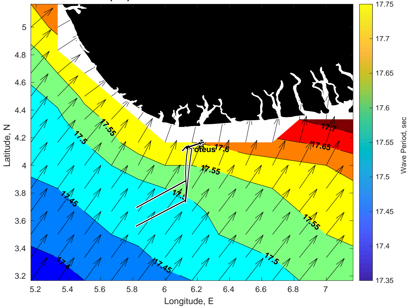
Wave Period (sec) for Proteus at 18-Feb-2025 09:00:00
