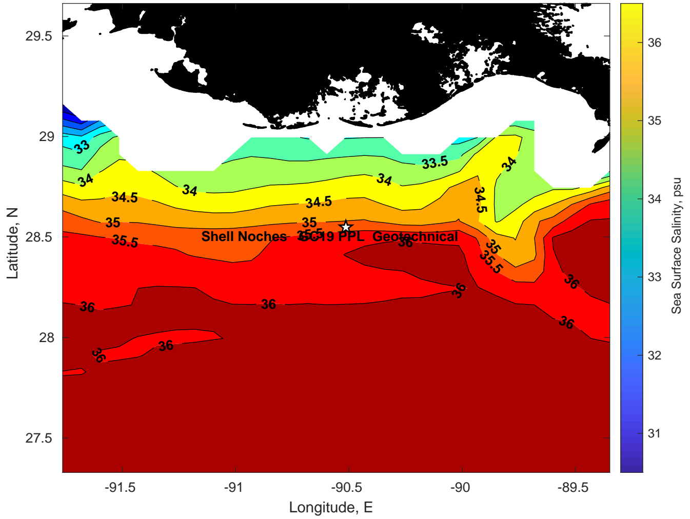
Surface Salinity for Shell Noches GC19 PPL Geotechnical at 17-Feb-2025 00:00:00
