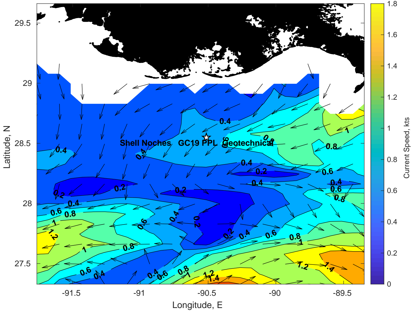
Surface Currents for Shell Noches GC19 PPL Geotechnical at 17-Feb-2025 00:00:00
