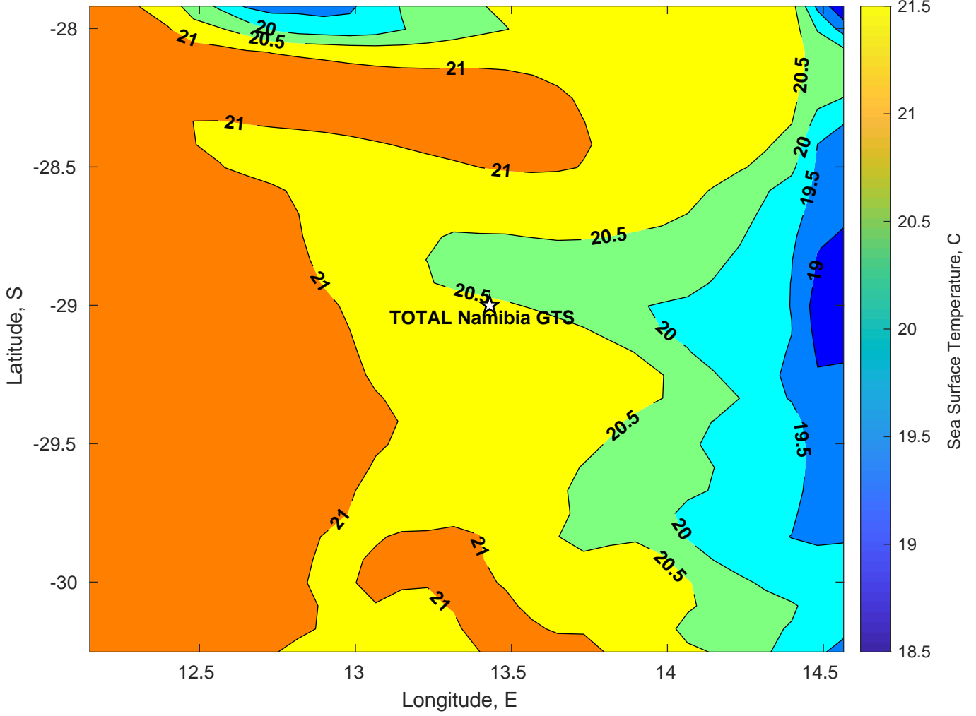
SST for TOTAL Namibia GTS at 17-Feb-2025 00:00:00
