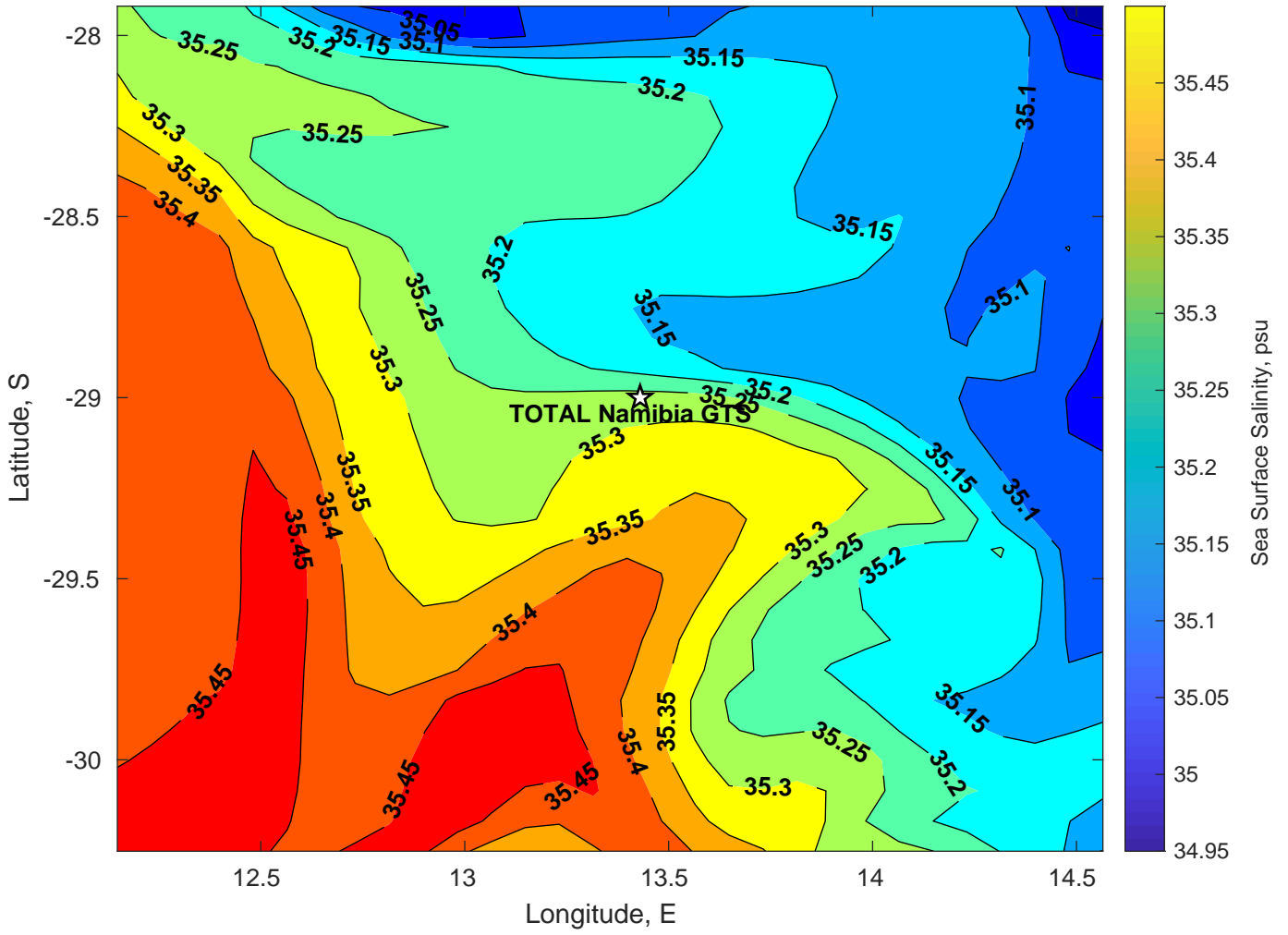
Surface Salinity for TOTAL Namibia GTS at 17-Feb-2025 00:00:00
