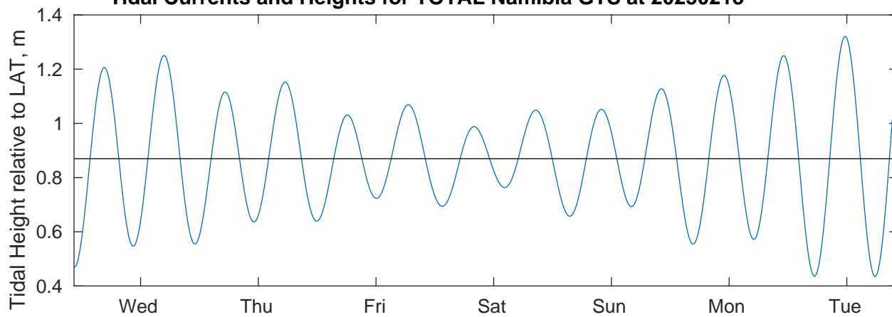
Tidal Currents and Heights for TOTAL Namibia GTS at 20250218
