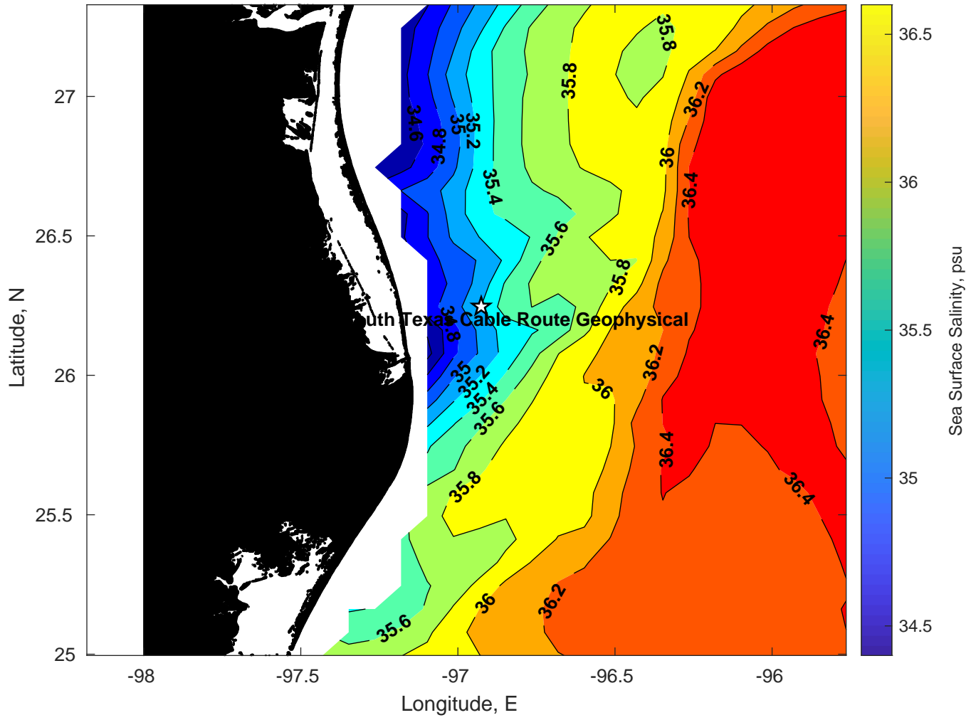
Surface Salinity for Tampnet P2378 South Texas Cable Route Geophysical at 17-Feb-2025 00:00:00
