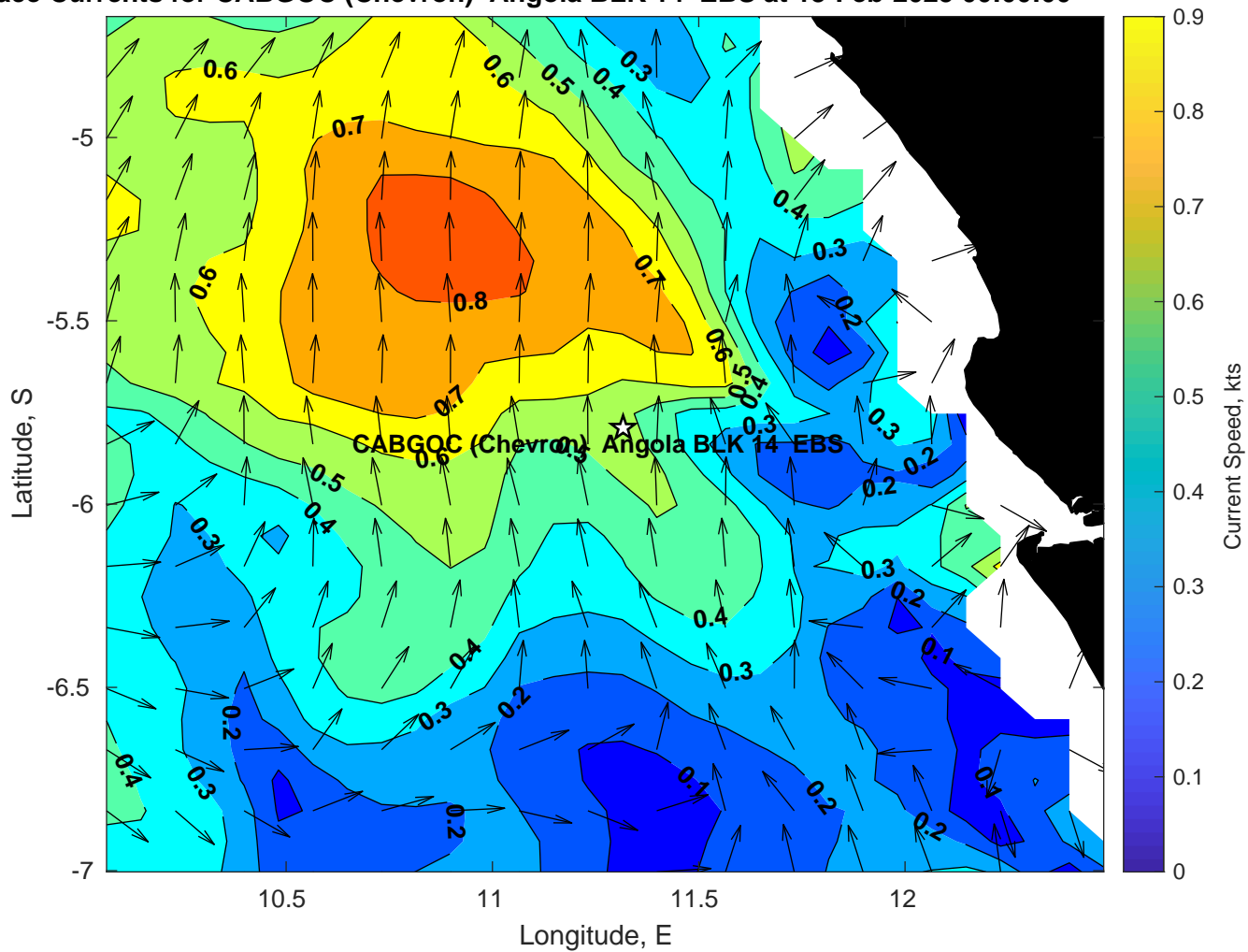
Surface Currents for CABGOC (Chevron) Angola BLK 14 EBS at 18-Feb-2025 00:00:00
