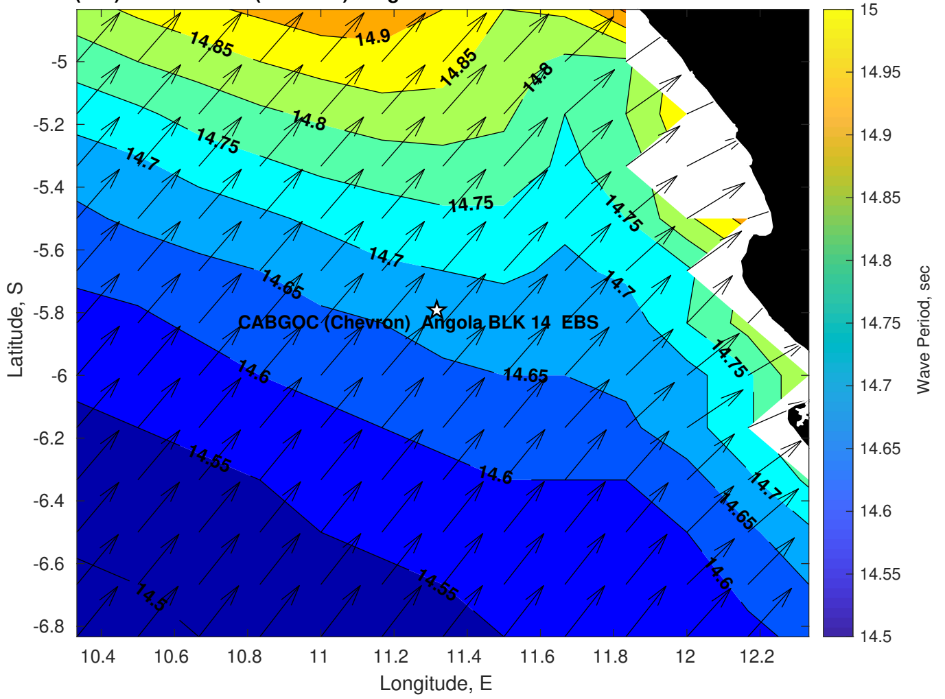
Wave Period (sec) for CABGOC (Chevron) Angola BLK 14 EBS at 19-Feb-2025 09:00:00
