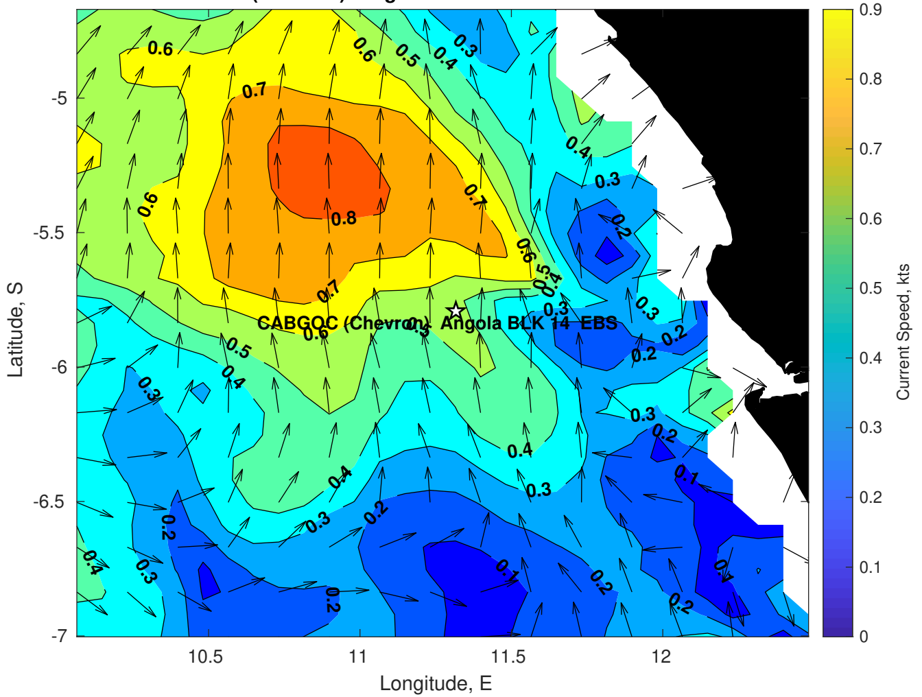
Surface Currents for CABGOC (Chevron) Angola BLK 14 EBS at 18-Feb-2025 00:00:00
