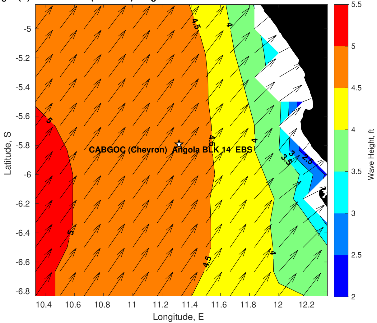
Wave Height (ft) for CABGOC (Chevron) Angola BLK 14 EBS at 19-Feb-2025 09:00:00
