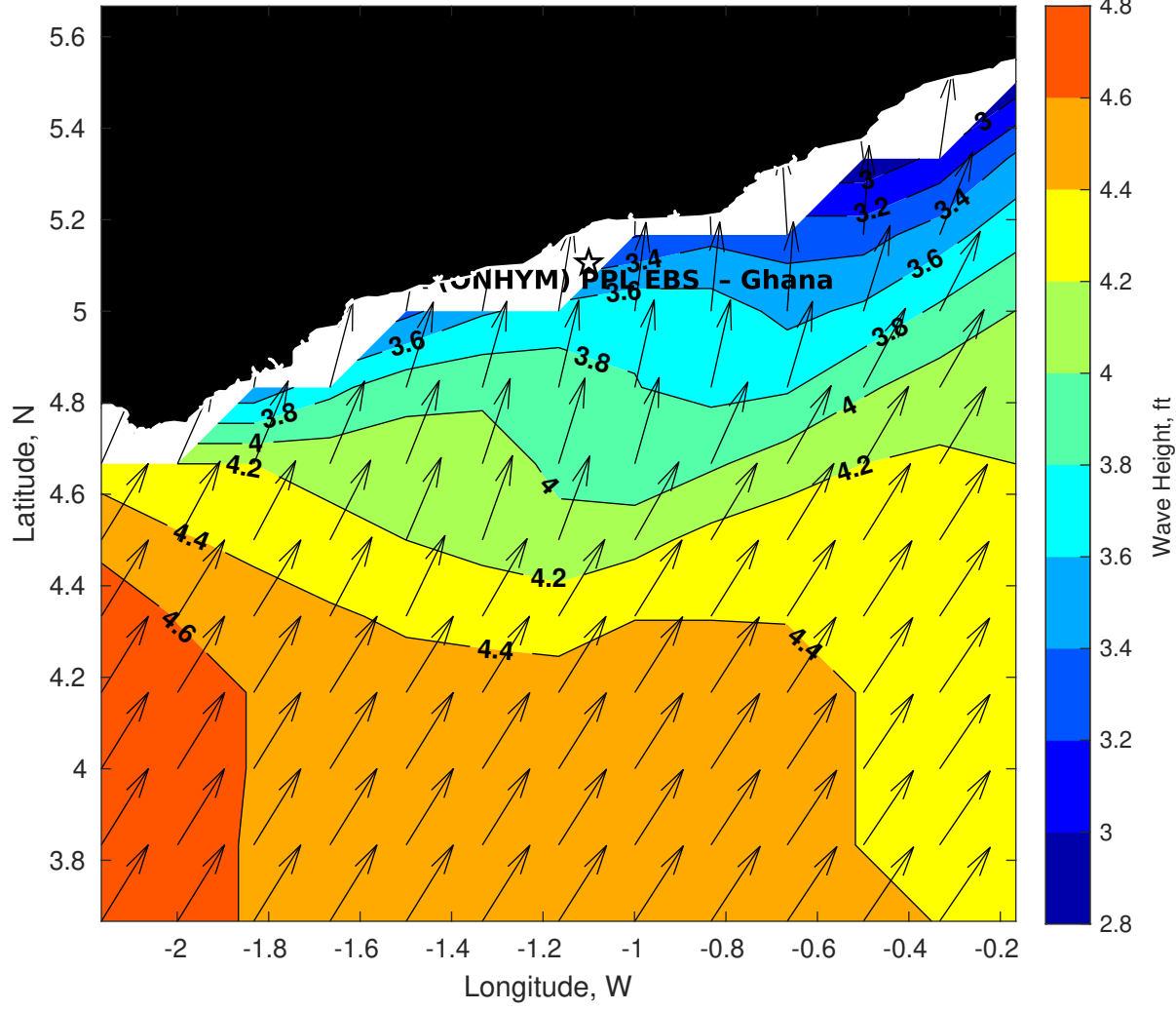
Wave Height (ft) for CSA (ONHYM) PPL EBS - Ghana at 19-Feb-2025 09:00:00
