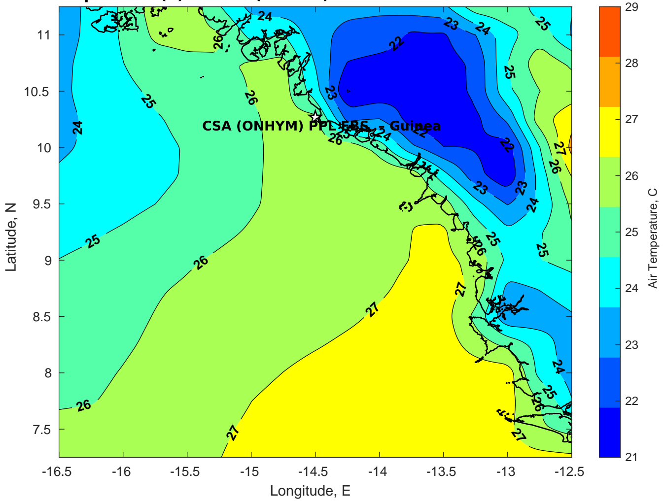
Air Temperature (C) for CSA (ONHYM) PPL EBS - Guinea at 19-Feb-2025
