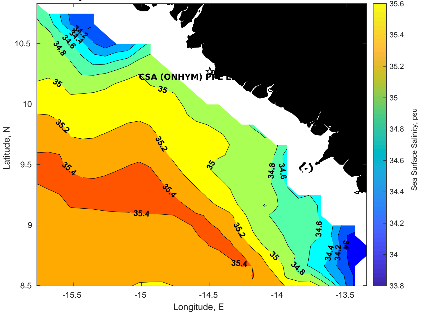
Surface Salinity for CSA (ONHYM) PPL EBS - Guinea at 18-Feb-2025 00:00:00
